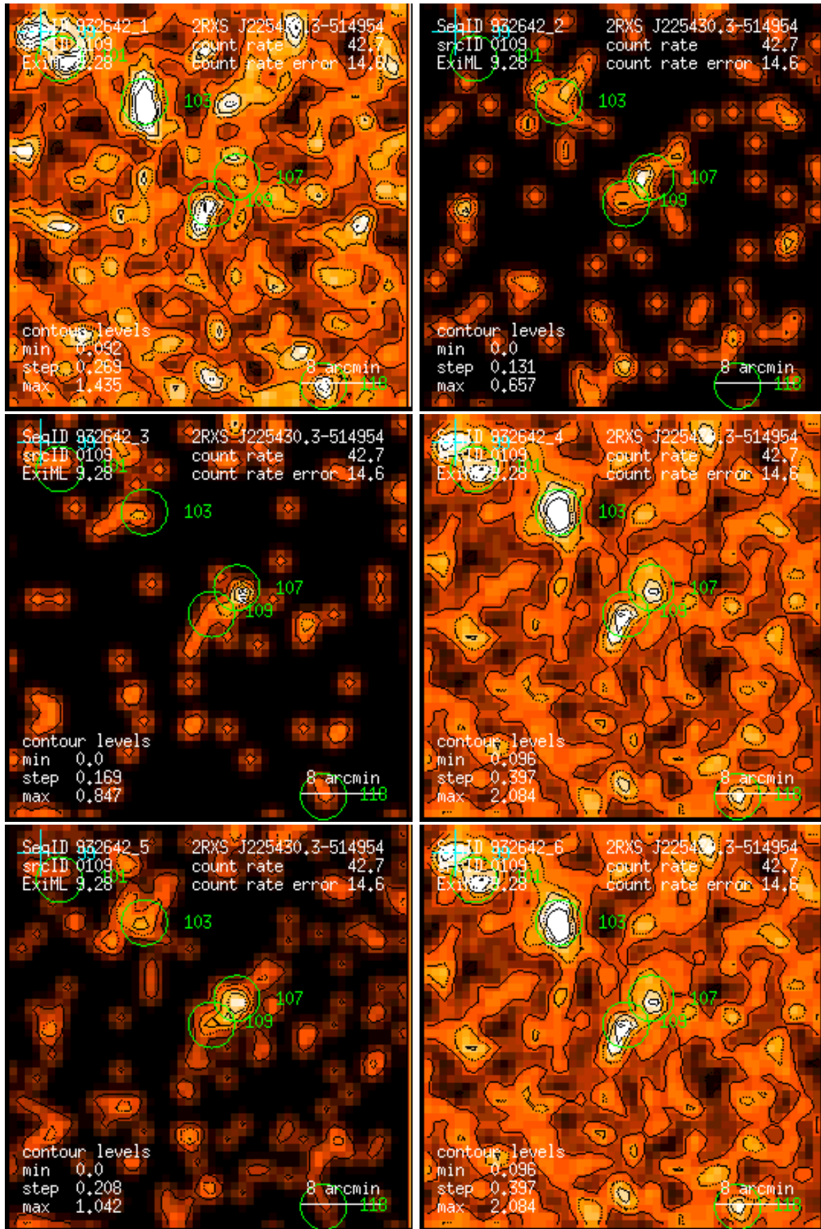
Figure 109: RASS 932642: detection 0109: band rate images, Gaussian filter: (1) PSPC channels 11 – 41, (2) 52 – 90, (3) 91 – 201, (4) 11 – 235, (5) 52 – 201, (6) 11 – 201. Broad band rates in counts/ks. Band rate contour levels in counts/ks/arcmin 2 .
