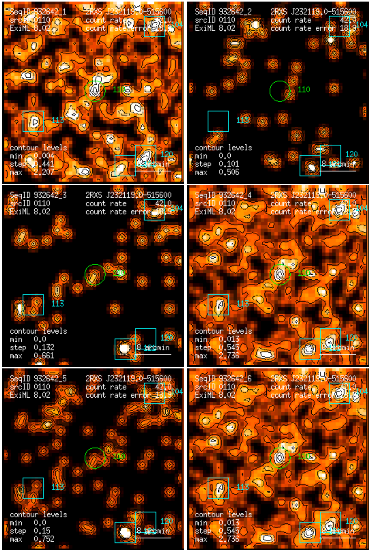
Figure 110: RASS 932642: detection 0110: band rate images, Gaussian filter: (1) PSPC channels 11 – 41, (2) 52 – 90, (3) 91 – 201, (4) 11 – 235, (5) 52 – 201, (6) 11 – 201. Broad band rates in counts/ks. Band rate contour levels in counts/ks/arcmin 2 .
