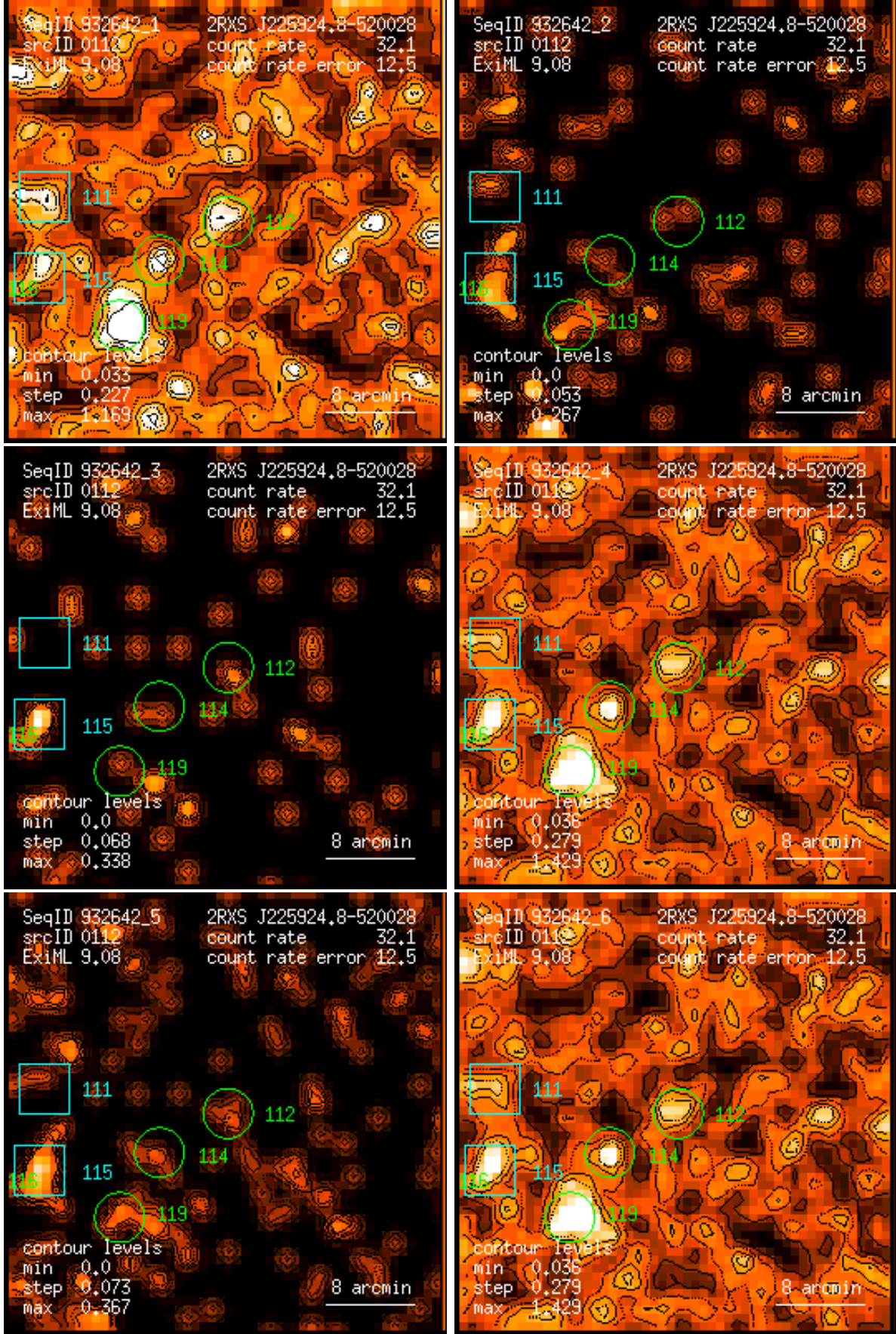
Figure 112: RASS 932642: detection 0112: band rate images, Gaussian filter: (1) PSPC channels 11 – 41, (2) 52 – 90, (3) 91 – 201, (4) 11 – 235, (5) 52 – 201, (6) 11 – 201. Broad band rates in counts/ks. Band rate contour levels in counts/ks/arcmin 2 .
