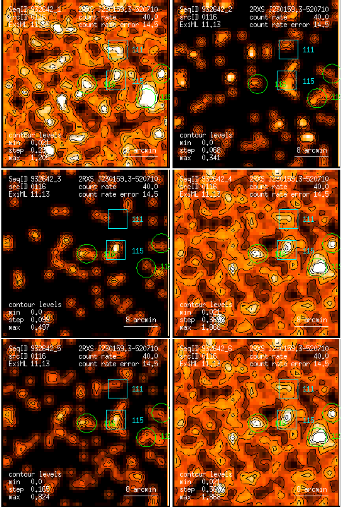
Figure 116: RASS 932642: detection 0116: band rate images, Gaussian filter: (1) PSPC channels 11 – 41, (2) 52 – 90, (3) 91 – 201, (4) 11 – 235, (5) 52 – 201, (6) 11 – 201. Broad band rates in counts/ks. Band rate contour levels in counts/ks/arcmin 2 .
