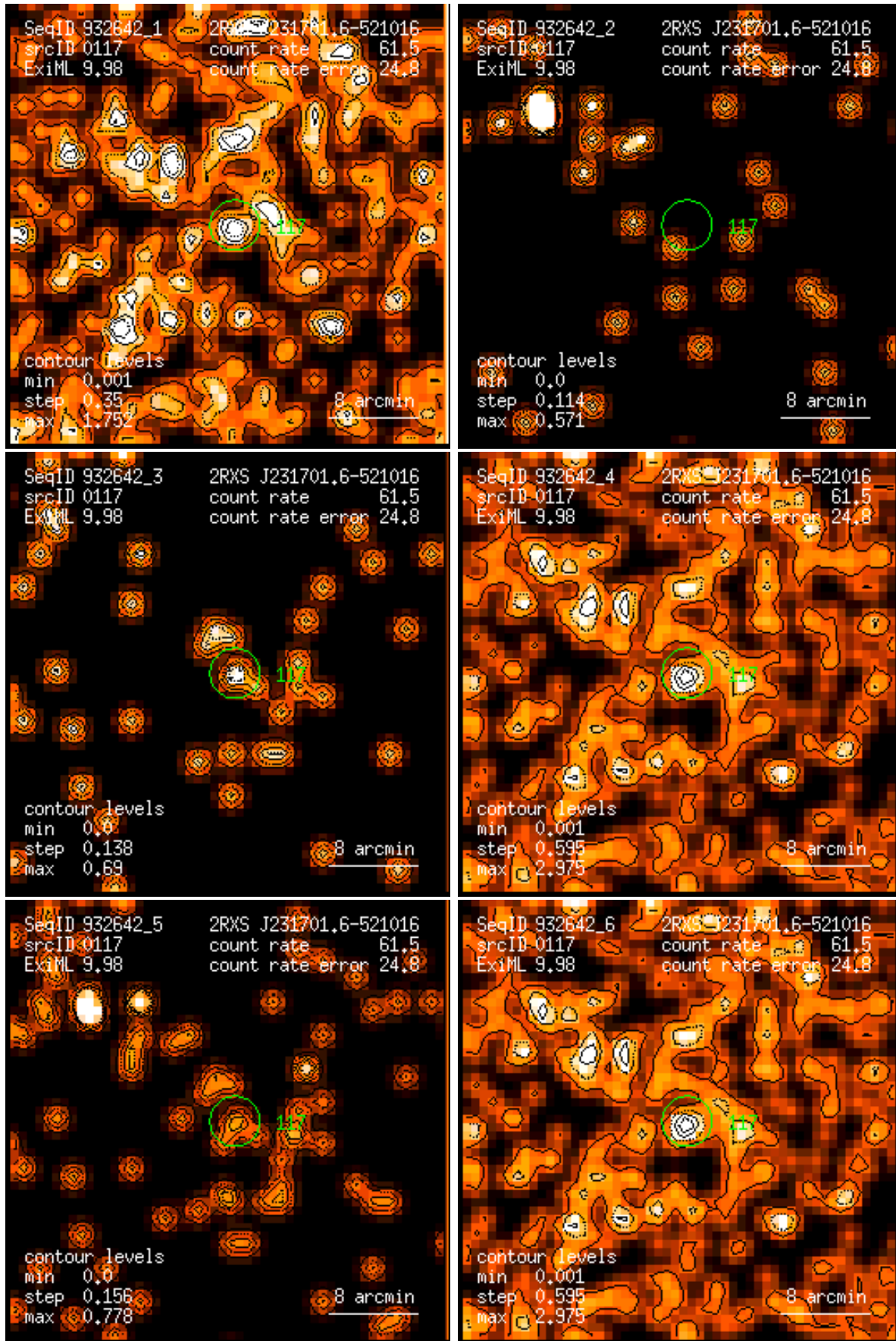
Figure 117: RASS 932642: detection 0117: band rate images, Gaussian filter: (1) PSPC channels 11 – 41, (2) 52 – 90, (3) 91 – 201, (4) 11 – 235, (5) 52 – 201, (6) 11 – 201. Broad band rates in counts/ks. Band rate contour levels in counts/ks/arcmin 2 .
