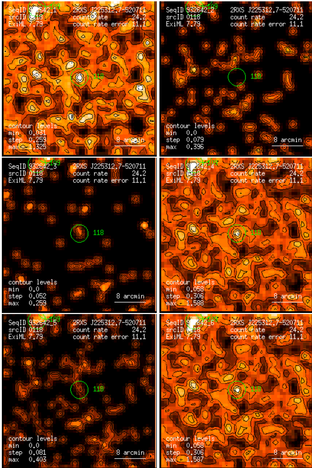
Figure 118: RASS 932642: detection 0118: band rate images, Gaussian filter: (1) PSPC channels 11 – 41, (2) 52 – 90, (3) 91 – 201, (4) 11 – 235, (5) 52 – 201, (6) 11 – 201. Broad band rates in counts/ks. Band rate contour levels in counts/ks/arcmin 2 .
