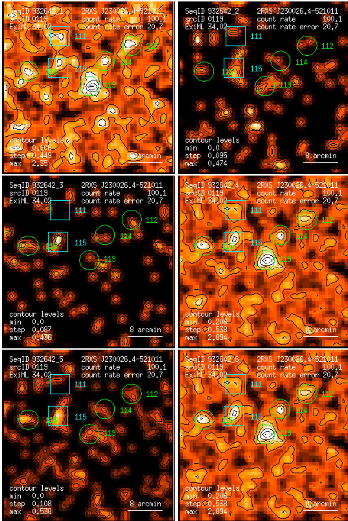
Figure 119: RASS 932642: detection 0119: band rate images, Gaussian filter: (1) PSPC channels 11 – 41, (2) 52 – 90, (3) 91 – 201, (4) 11 – 235, (5) 52 – 201, (6) 11 – 201. Broad band rates in counts/ks. Band rate contour levels in counts/ks/arcmin 2 .
