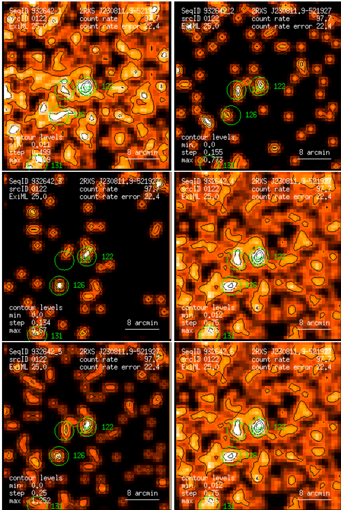
Figure 122: RASS 932642: detection 0122: band rate images, Gaussian filter: (1) PSPC channels 11 – 41, (2) 52 – 90, (3) 91 – 201, (4) 11 – 235, (5) 52 – 201, (6) 11 – 201. Broad band rates in counts/ks. Band rate contour levels in counts/ks/arcmin 2 .
