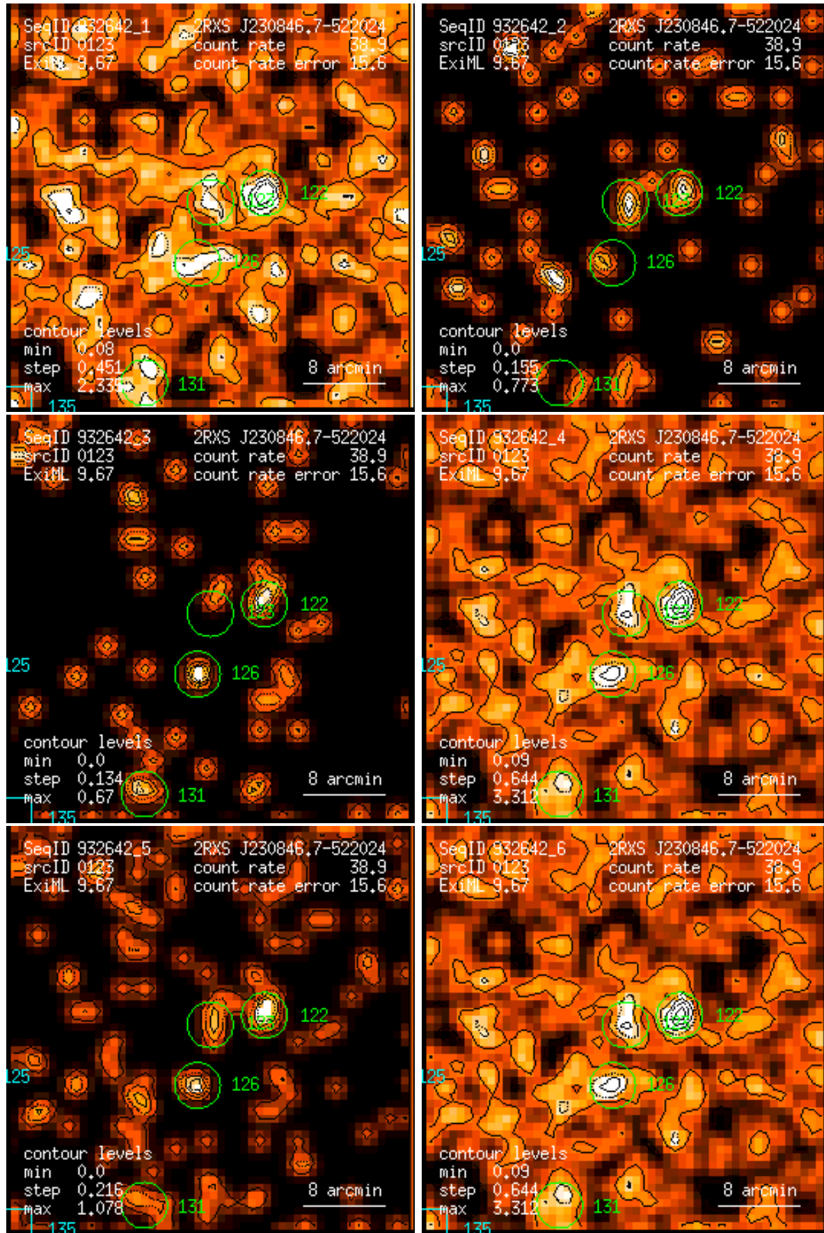
Figure 123: RASS 932642: detection 0123: band rate images, Gaussian filter: (1) PSPC channels 11 – 41, (2) 52 – 90, (3) 91 – 201, (4) 11 – 235, (5) 52 – 201, (6) 11 – 201. Broad band rates in counts/ks. Band rate contour levels in counts/ks/arcmin 2 .
