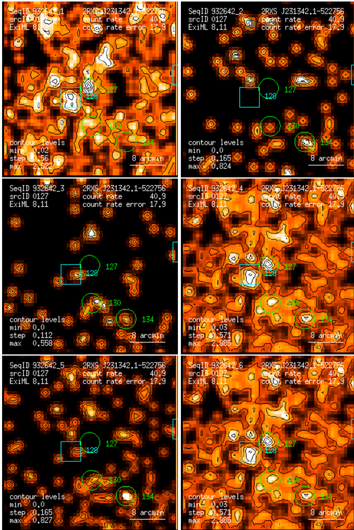
Figure 127: RASS 932642: detection 0127: band rate images, Gaussian filter: (1) PSPC channels 11 – 41, (2) 52 – 90, (3) 91 – 201, (4) 11 – 235, (5) 52 – 201, (6) 11 – 201. Broad band rates in counts/ks. Band rate contour levels in counts/ks/arcmin 2 .
