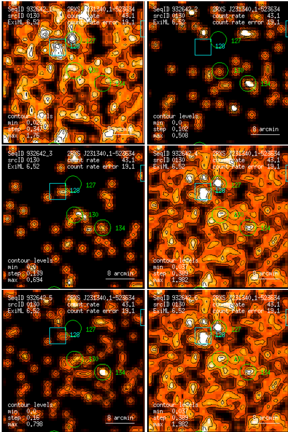
Figure 130: RASS 932642: detection 0130: band rate images, Gaussian filter: (1) PSPC channels 11 – 41, (2) 52 – 90, (3) 91 – 201, (4) 11 – 235, (5) 52 – 201, (6) 11 – 201. Broad band rates in counts/ks. Band rate contour levels in counts/ks/arcmin 2 .
