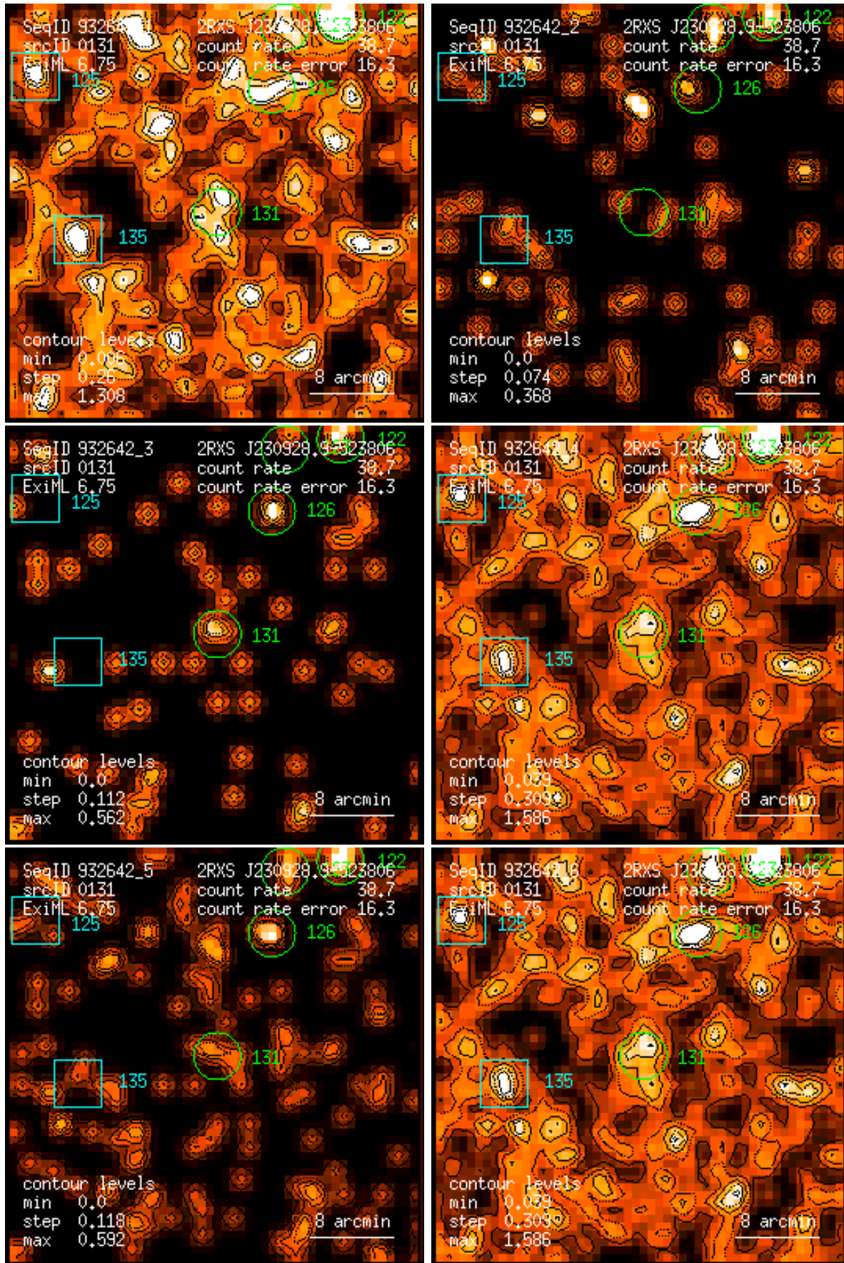
Figure 131: RASS 932642: detection 0131: band rate images, Gaussian filter: (1) PSPC channels 11 – 41, (2) 52 – 90, (3) 91 – 201, (4) 11 – 235, (5) 52 – 201, (6) 11 – 201. Broad band rates in counts/ks. Band rate contour levels in counts/ks/arcmin 2 .
