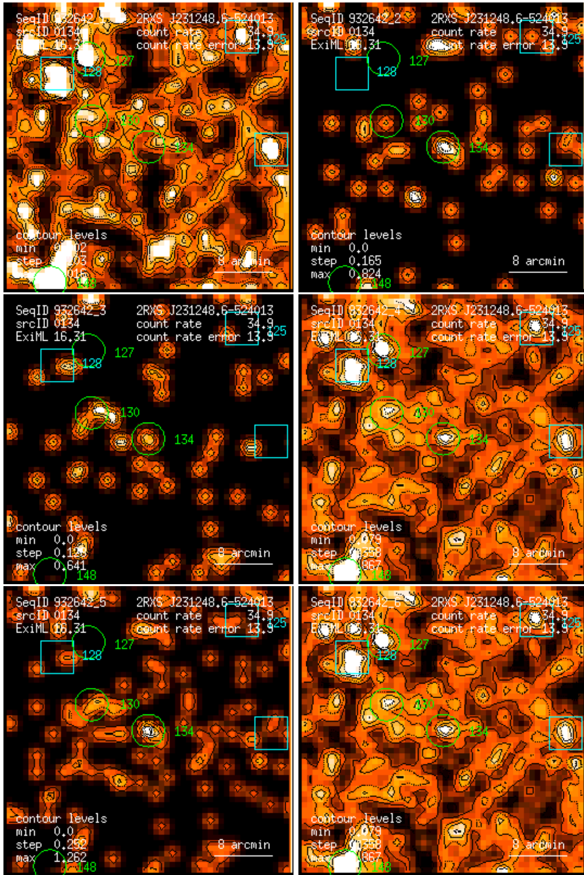
Figure 134: RASS 932642: detection 0134: band rate images, Gaussian filter: (1) PSPC channels 11 – 41, (2) 52 – 90, (3) 91 – 201, (4) 11 – 235, (5) 52 – 201, (6) 11 – 201. Broad band rates in counts/ks. Band rate contour levels in counts/ks/arcmin 2 .
