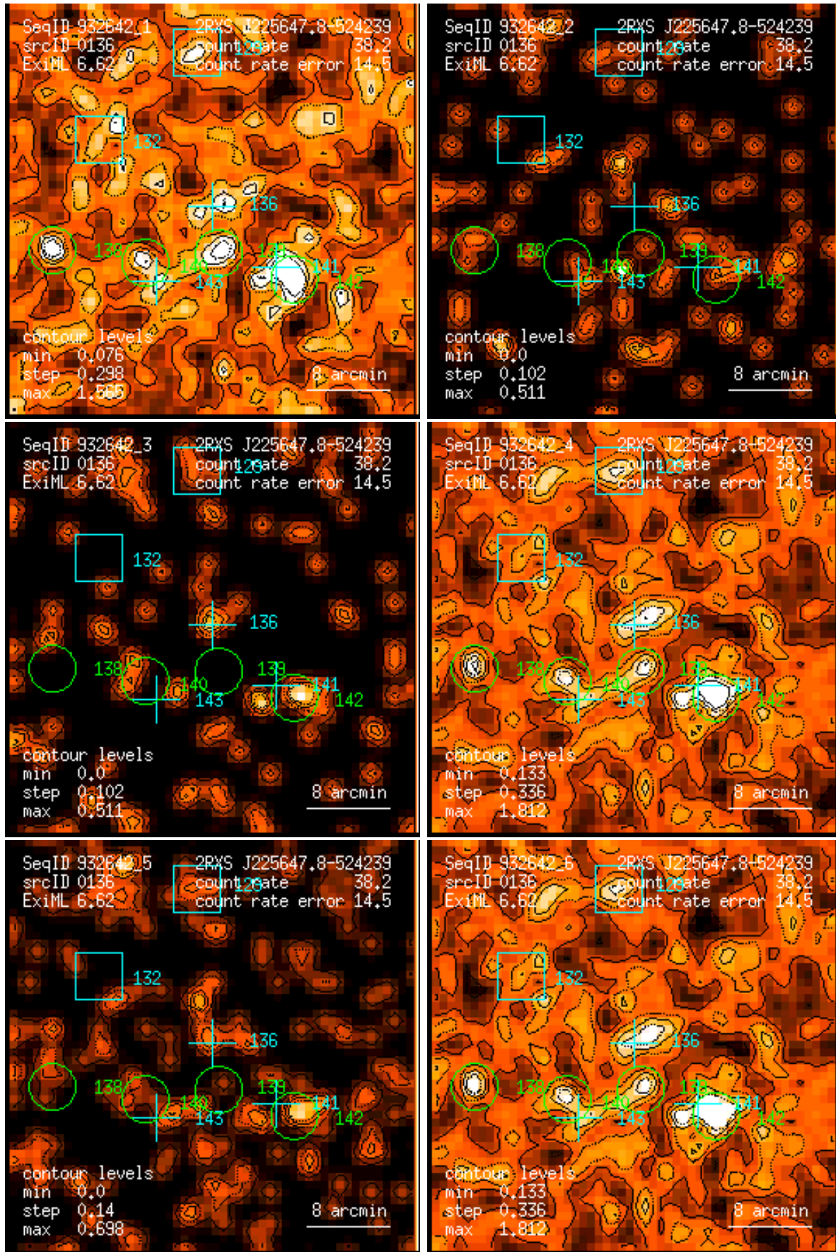
Figure 136: RASS 932642: detection 0136: band rate images, Gaussian filter: (1) PSPC channels 11 – 41, (2) 52 – 90, (3) 91 – 201, (4) 11 – 235, (5) 52 – 201, (6) 11 – 201. Broad band rates in counts/ks. Band rate contour levels in counts/ks/arcmin 2 .
