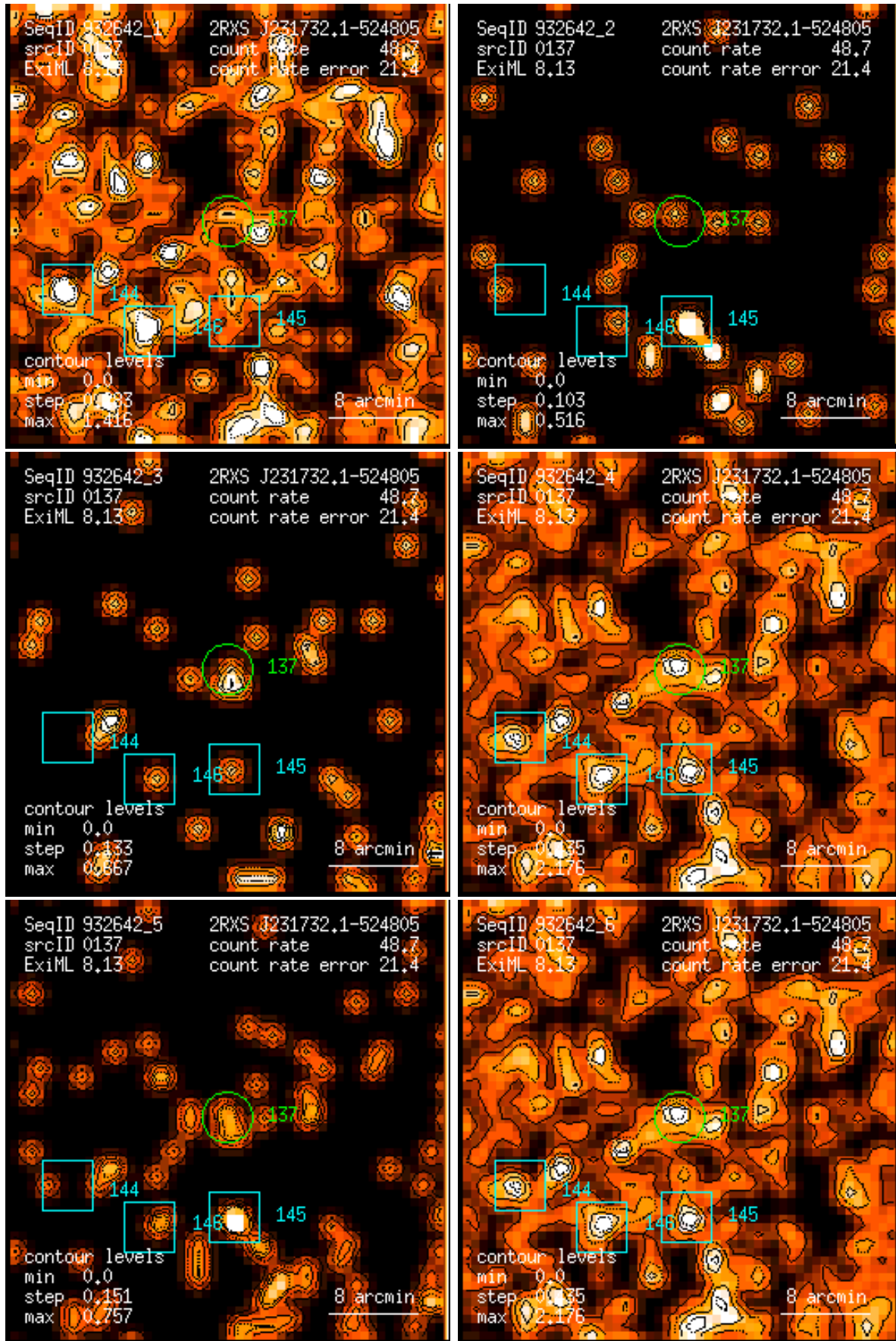
Figure 137: RASS 932642: detection 0137: band rate images, Gaussian filter: (1) PSPC channels 11 – 41, (2) 52 – 90, (3) 91 – 201, (4) 11 – 235, (5) 52 – 201, (6) 11 – 201. Broad band rates in counts/ks. Band rate contour levels in counts/ks/arcmin 2 .
