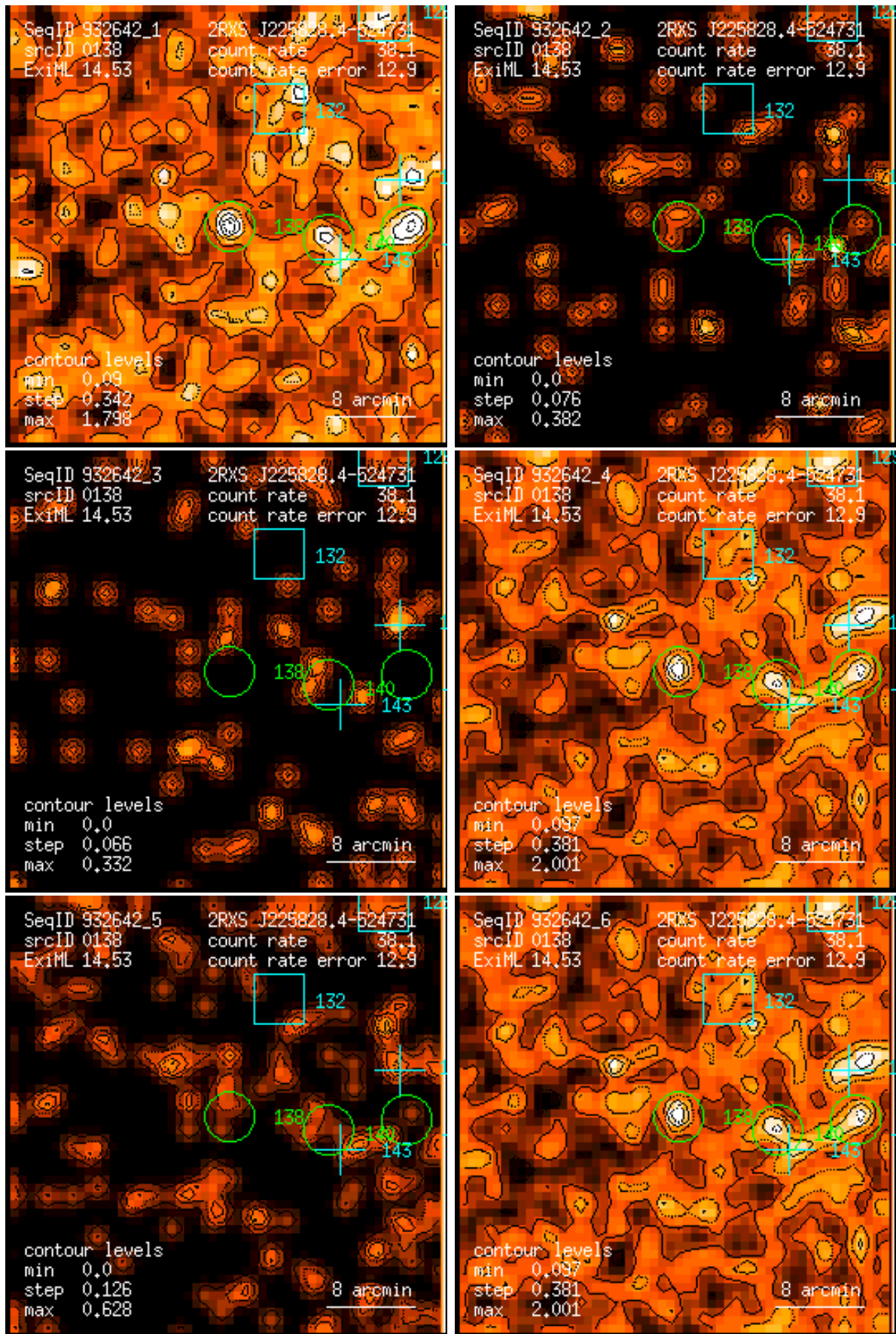
Figure 138: RASS 932642: detection 0138: band rate images, Gaussian filter: (1) PSPC channels 11 – 41, (2) 52 – 90, (3) 91 – 201, (4) 11 – 235, (5) 52 – 201, (6) 11 – 201. Broad band rates in counts/ks. Band rate contour levels in counts/ks/arcmin 2 .
