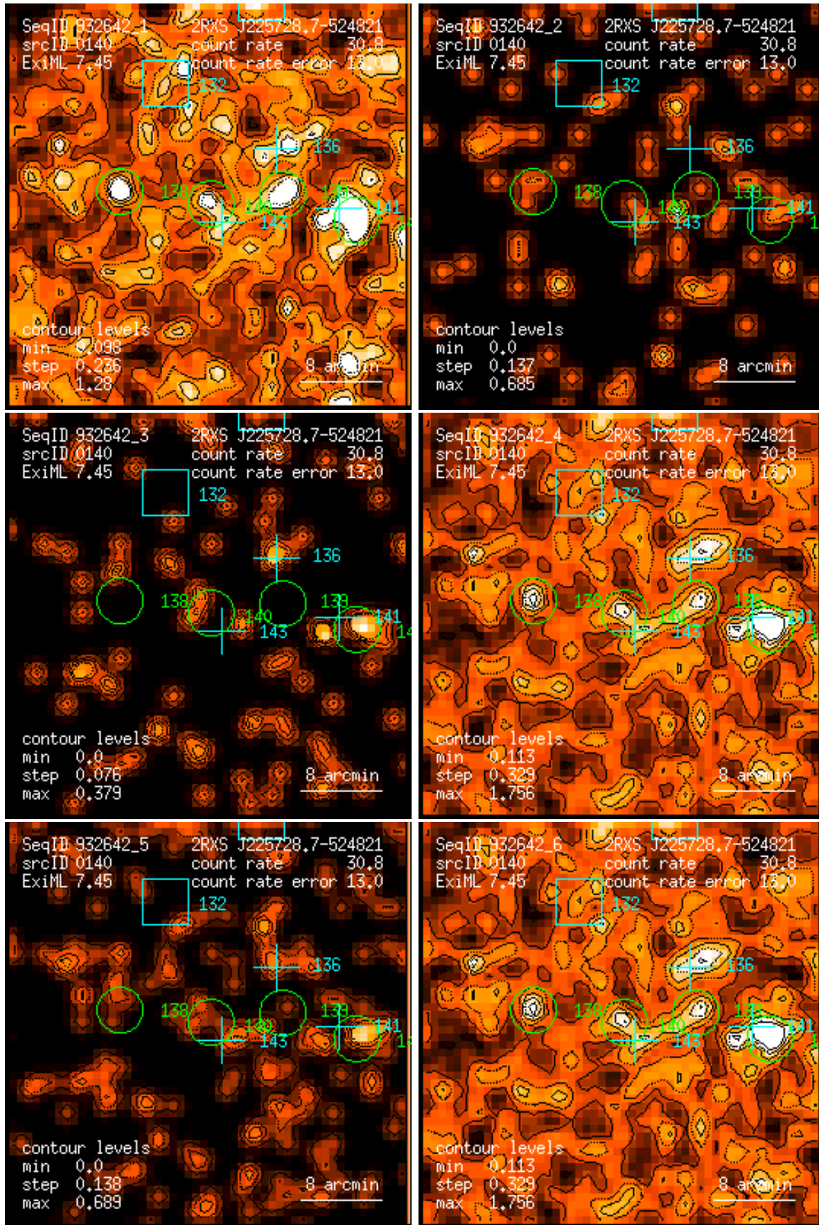
Figure 140: RASS 932642: detection 0140: band rate images, Gaussian filter: (1) PSPC channels 11 – 41, (2) 52 – 90, (3) 91 – 201, (4) 11 – 235, (5) 52 – 201, (6) 11 – 201. Broad band rates in counts/ks. Band rate contour levels in counts/ks/arcmin 2 .
