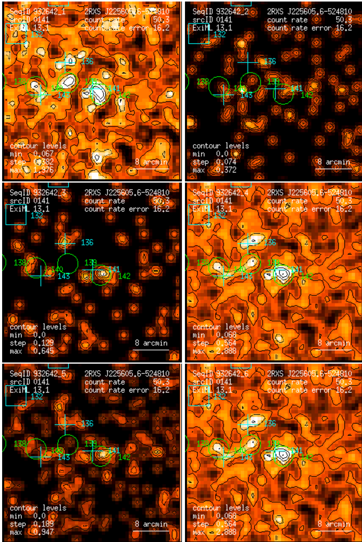
Figure 141: RASS 932642: detection 0141: band rate images, Gaussian filter: (1) PSPC channels 11 – 41, (2) 52 – 90, (3) 91 – 201, (4) 11 – 235, (5) 52 – 201, (6) 11 – 201. Broad band rates in counts/ks. Band rate contour levels in counts/ks/arcmin 2 .
