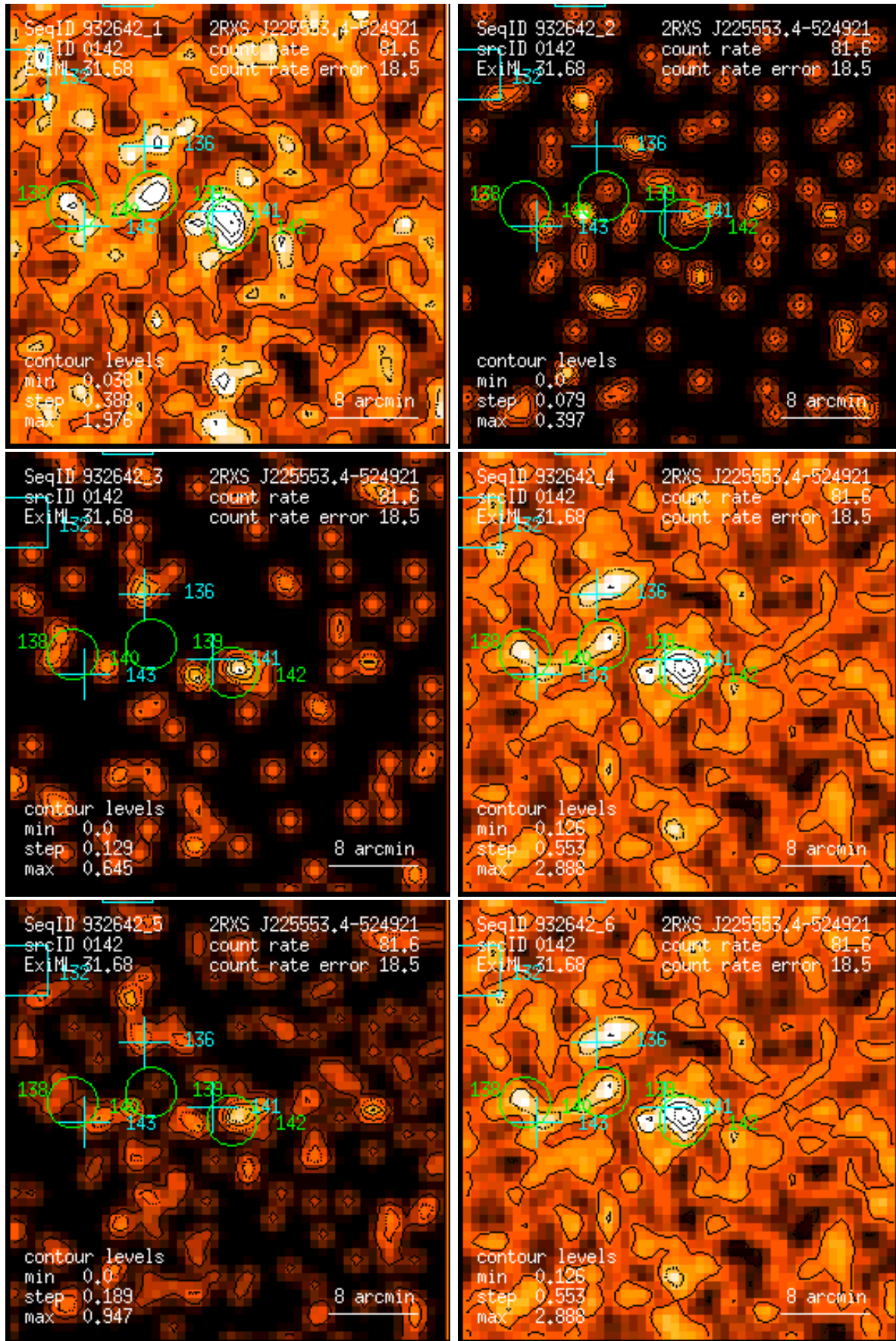
Figure 142: RASS 932642: detection 0142: band rate images, Gaussian filter: (1) PSPC channels 11 – 41, (2) 52 – 90, (3) 91 – 201, (4) 11 – 235, (5) 52 – 201, (6) 11 – 201. Broad band rates in counts/ks. Band rate contour levels in counts/ks/arcmin 2 .
