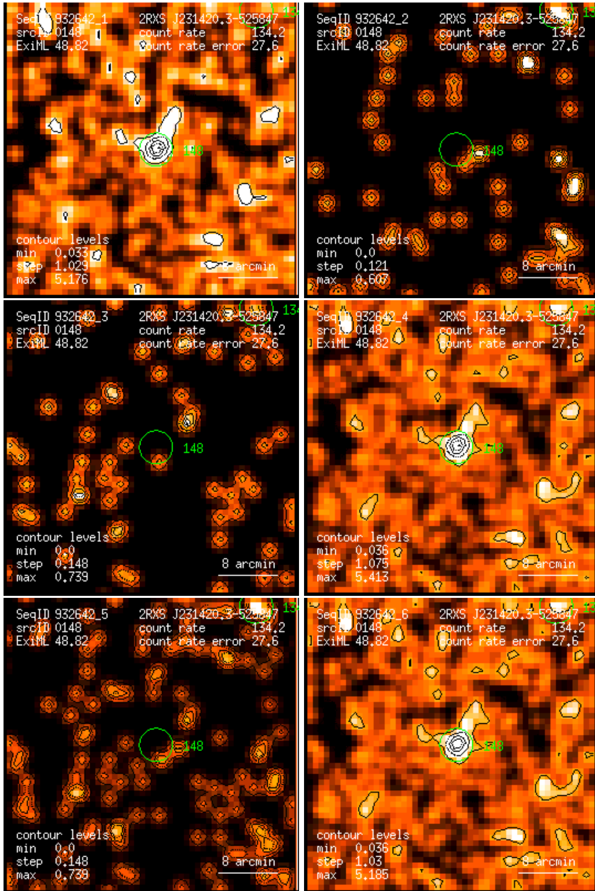
Figure 148: RASS 932642: detection 0148: band rate images, Gaussian filter: (1) PSPC channels 11 – 41, (2) 52 – 90, (3) 91 – 201, (4) 11 – 235, (5) 52 – 201, (6) 11 – 201. Broad band rates in counts/ks. Band rate contour levels in counts/ks/arcmin 2 .
