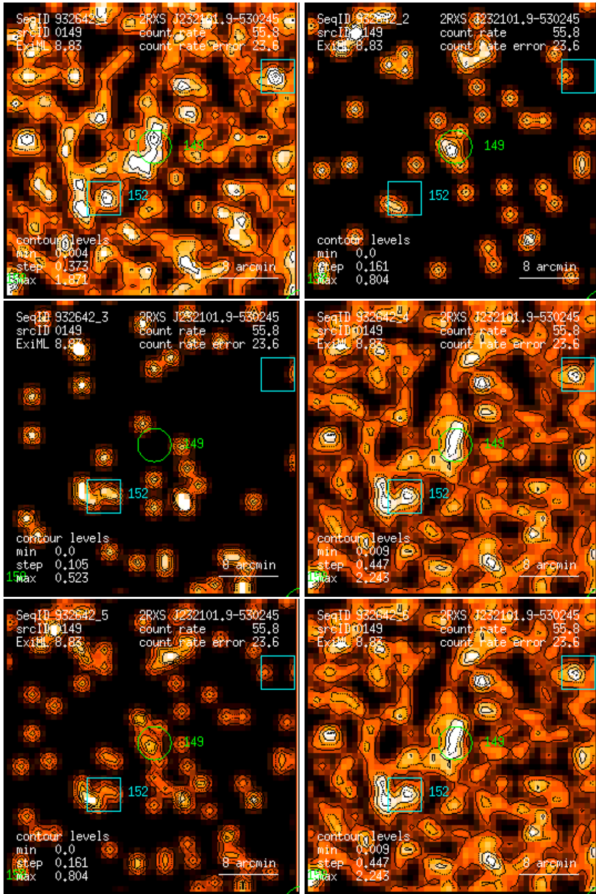
Figure 149: RASS 932642: detection 0149: band rate images, Gaussian filter: (1) PSPC channels 11 – 41, (2) 52 – 90, (3) 91 – 201, (4) 11 – 235, (5) 52 – 201, (6) 11 – 201. Broad band rates in counts/ks. Band rate contour levels in counts/ks/arcmin 2 .
