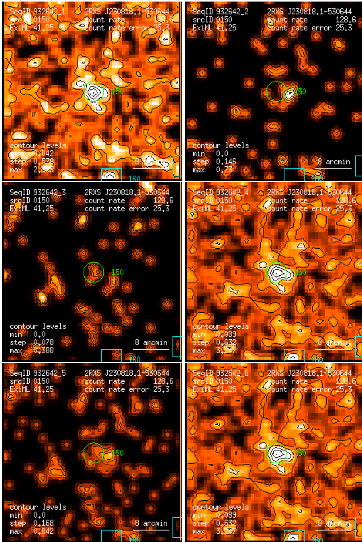
Figure 150: RASS 932642: detection 0150: band rate images, Gaussian filter: (1) PSPC channels 11 – 41, (2) 52 – 90, (3) 91 – 201, (4) 11 – 235, (5) 52 – 201, (6) 11 – 201. Broad band rates in counts/ks. Band rate contour levels in counts/ks/arcmin 2 .
