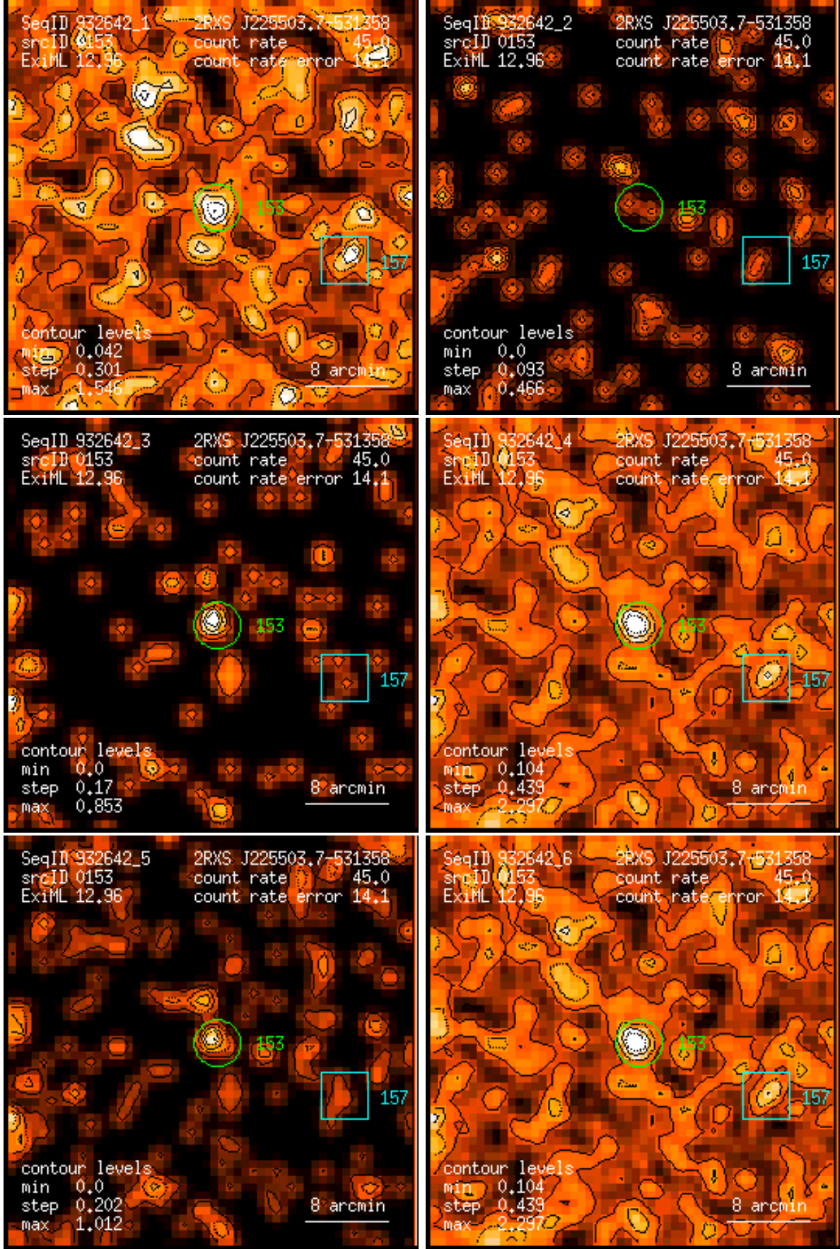
Figure 153: RASS 932642: detection 0153: band rate images, Gaussian filter: (1) PSPC channels 11 – 41, (2) 52 – 90, (3) 91 – 201, (4) 11 – 235, (5) 52 – 201, (6) 11 – 201. Broad band rates in counts/ks. Band rate contour levels in counts/ks/arcmin 2 .
