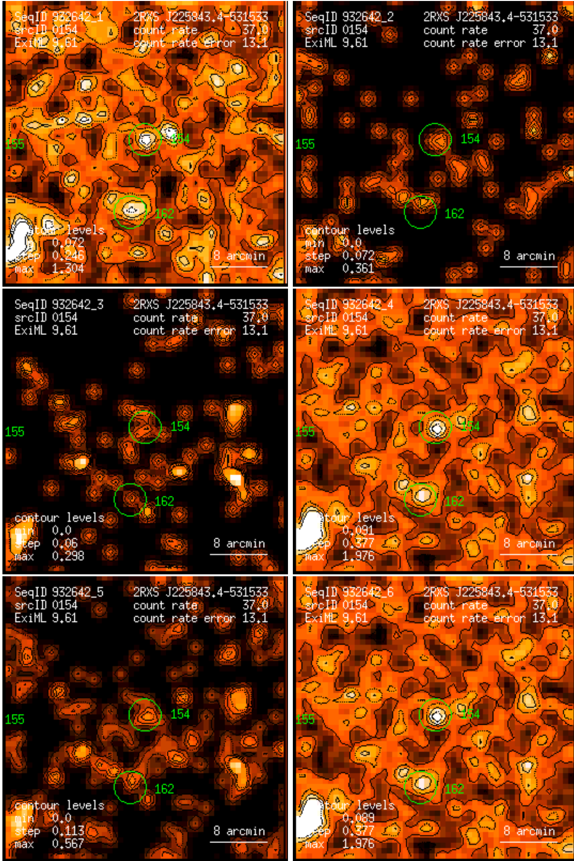
Figure 154: RASS 932642: detection 0154: band rate images, Gaussian filter: (1) PSPC channels 11 – 41, (2) 52 – 90, (3) 91 – 201, (4) 11 – 235, (5) 52 – 201, (6) 11 – 201. Broad band rates in counts/ks. Band rate contour levels in counts/ks/arcmin 2 .
