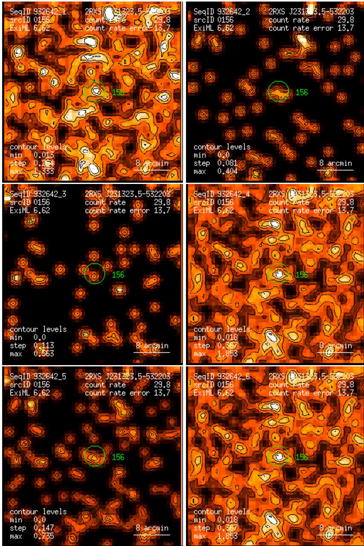
Figure 156: RASS 932642: detection 0156: band rate images, Gaussian filter: (1) PSPC channels 11 – 41, (2) 52 – 90, (3) 91 – 201, (4) 11 – 235, (5) 52 – 201, (6) 11 – 201. Broad band rates in counts/ks. Band rate contour levels in counts/ks/arcmin 2 .
