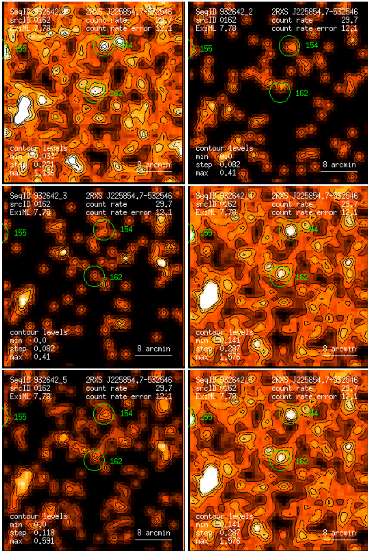
Figure 162: RASS 932642: detection 0162: band rate images, Gaussian filter: (1) PSPC channels 11 – 41, (2) 52 – 90, (3) 91 – 201, (4) 11 – 235, (5) 52 – 201, (6) 11 – 201. Broad band rates in counts/ks. Band rate contour levels in counts/ks/arcmin 2 .
