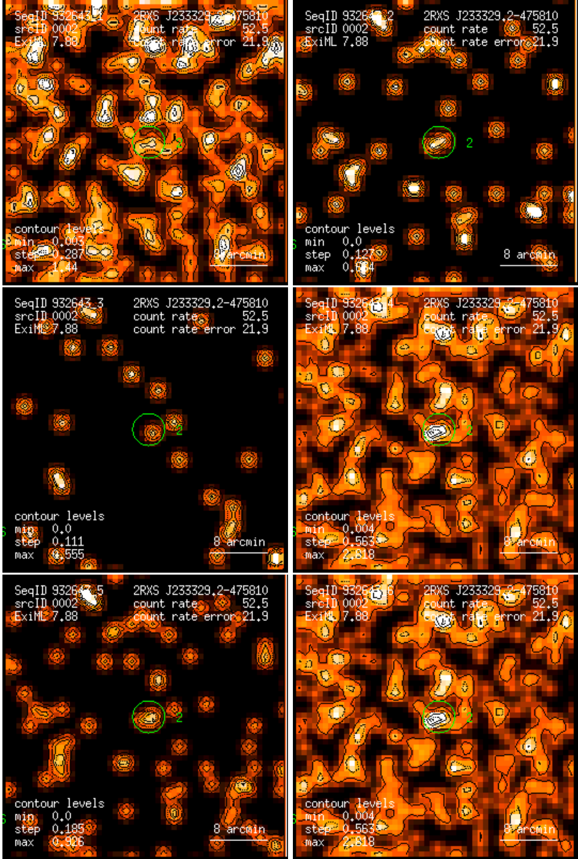
Figure 2: RASS 932643: detection 0002: band rate images, Gaussian filter: (1) PSPC channels 11 – 41, (2) 52 – 90, (3) 91 – 201, (4) 11 – 235, (5) 52 – 201, (6) 11 – 201. Broad band rates in counts/ks. Band rate contour levels in counts/ks/arcmin 2 .
