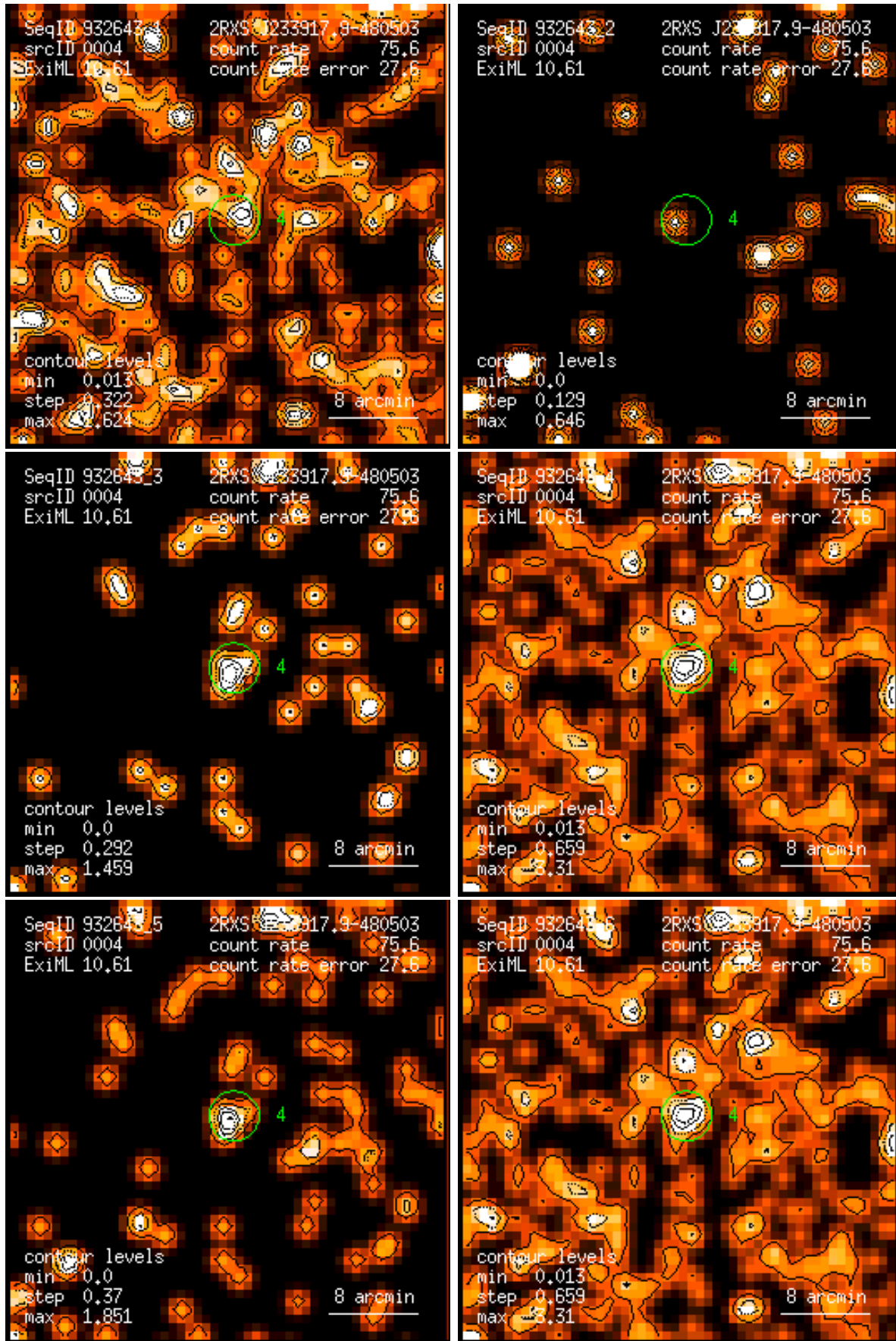
Figure 4: RASS 932643: detection 0004: band rate images, Gaussian filter: (1) PSPC channels 11 – 41, (2) 52 – 90, (3) 91 – 201, (4) 11 – 235, (5) 52 – 201, (6) 11 – 201. Broad band rates in counts/ks. Band rate contour levels in counts/ks/arcmin 2 .
