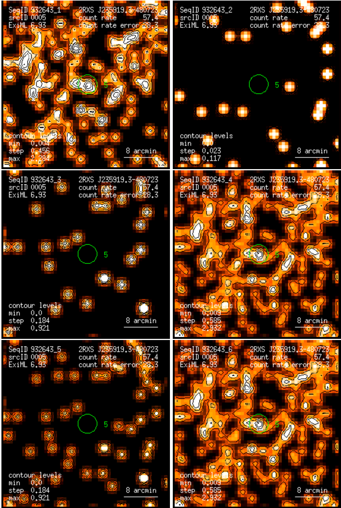
Figure 5: RASS 932643: detection 0005: band rate images, Gaussian filter: (1) PSPC channels 11 – 41, (2) 52 – 90, (3) 91 – 201, (4) 11 – 235, (5) 52 – 201, (6) 11 – 201. Broad band rates in counts/ks. Band rate contour levels in counts/ks/arcmin 2 .
