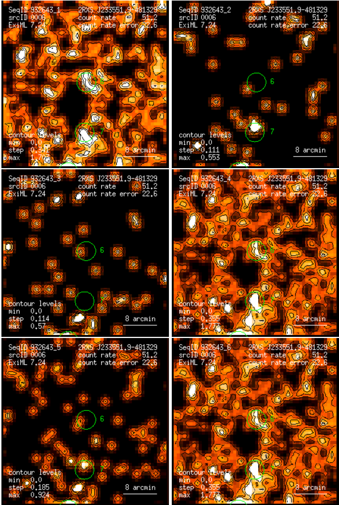
Figure 6: RASS 932643: detection 0006: band rate images, Gaussian filter: (1) PSPC channels 11 – 41, (2) 52 – 90, (3) 91 – 201, (4) 11 – 235, (5) 52 – 201, (6) 11 – 201. Broad band rates in counts/ks. Band rate contour levels in counts/ks/arcmin 2 .
