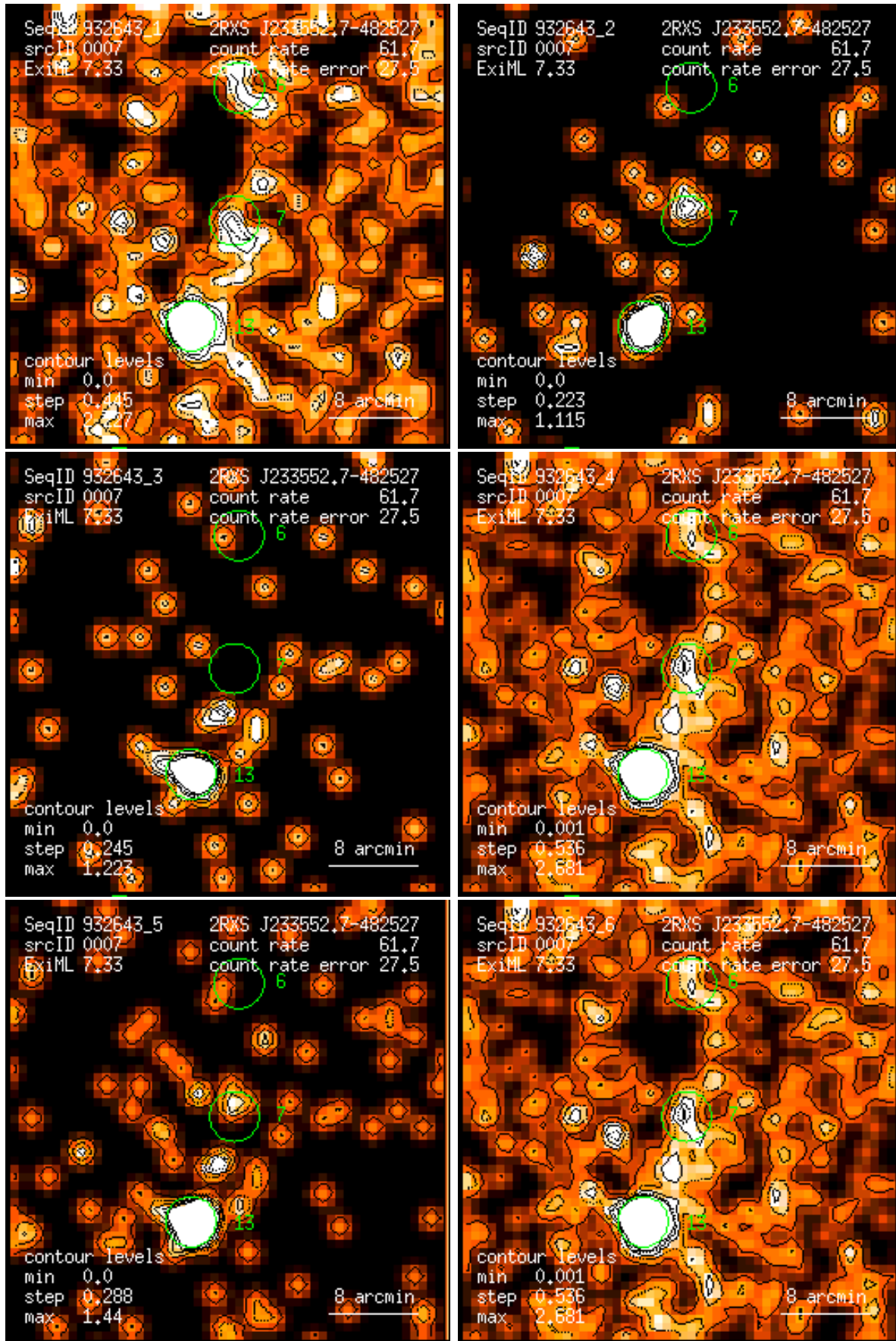
Figure 7: RASS 932643: detection 0007: band rate images, Gaussian filter: (1) PSPC channels 11 – 41, (2) 52 – 90, (3) 91 – 201, (4) 11 – 235, (5) 52 – 201, (6) 11 – 201. Broad band rates in counts/ks. Band rate contour levels in counts/ks/arcmin 2 .
