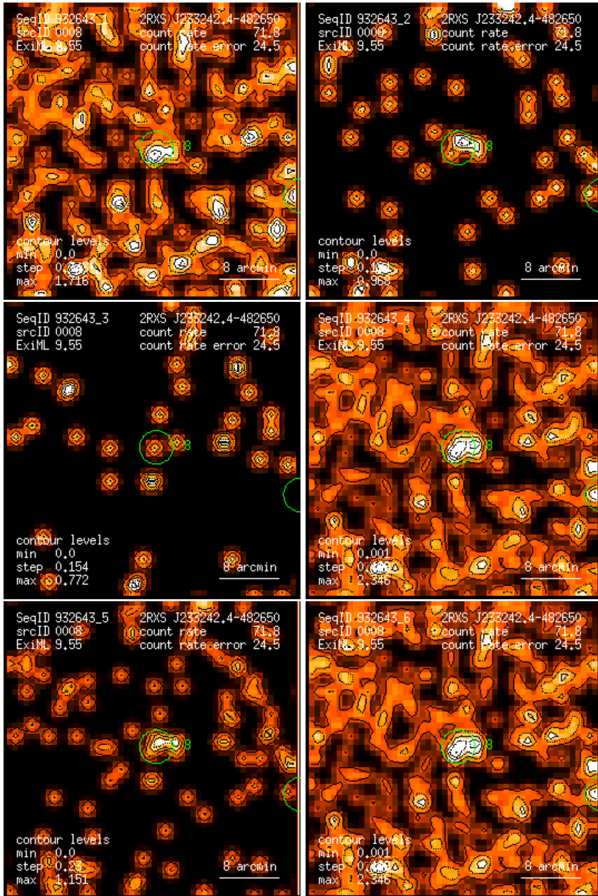
Figure 8: RASS 932643: detection 0008: band rate images, Gaussian filter: (1) PSPC channels 11 – 41, (2) 52 – 90, (3) 91 – 201, (4) 11 – 235, (5) 52 – 201, (6) 11 – 201. Broad band rates in counts/ks. Band rate contour levels in counts/ks/arcmin 2 .
