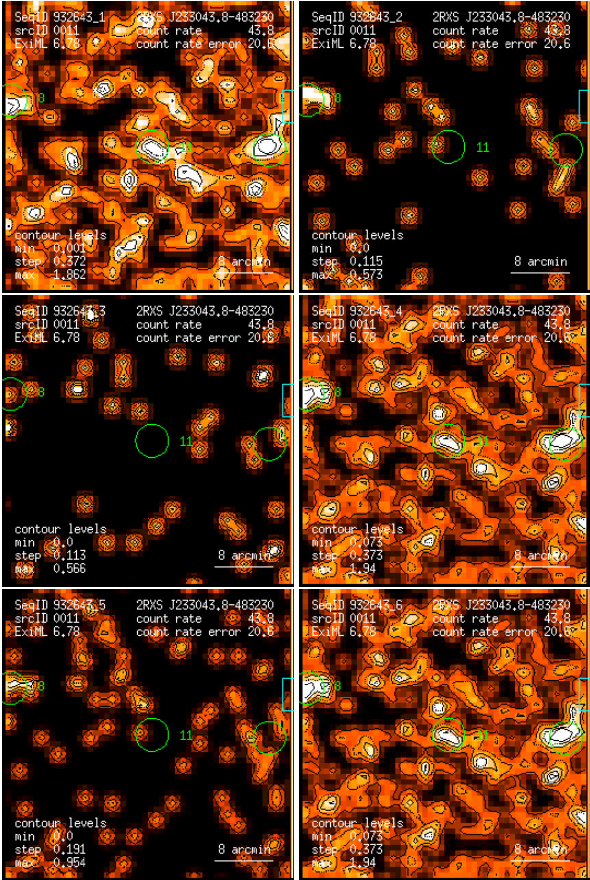
Figure 11: RASS 932643: detection 0011: band rate images, Gaussian filter: (1) PSPC channels 11 – 41, (2) 52 – 90, (3) 91 – 201, (4) 11 – 235, (5) 52 – 201, (6) 11 – 201. Broad band rates in counts/ks. Band rate contour levels in counts/ks/arcmin 2 .
