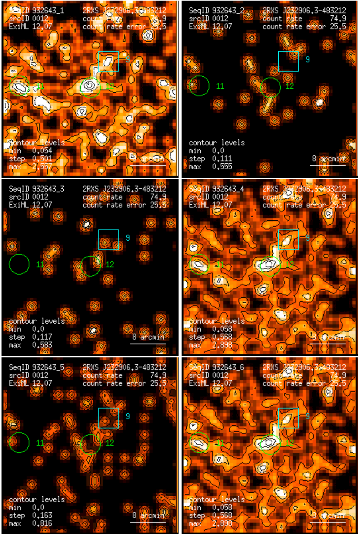
Figure 12: RASS 932643: detection 0012: band rate images, Gaussian filter: (1) PSPC channels 11 – 41, (2) 52 – 90, (3) 91 – 201, (4) 11 – 235, (5) 52 – 201, (6) 11 – 201. Broad band rates in counts/ks. Band rate contour levels in counts/ks/arcmin 2 .
