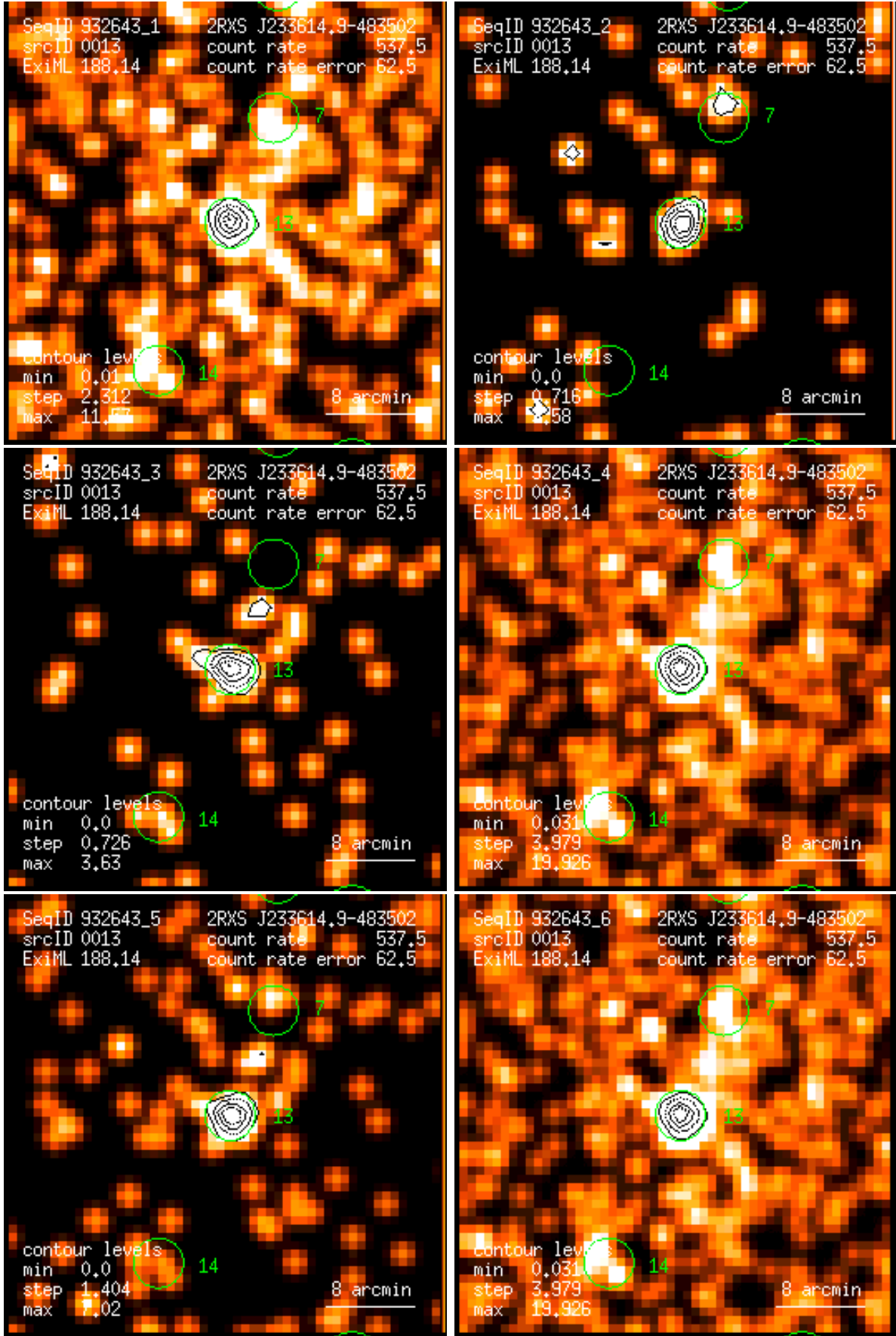
Figure 13: RASS 932643: detection 0013: band rate images, Gaussian filter: (1) PSPC channels 11 – 41, (2) 52 – 90, (3) 91 – 201, (4) 11 – 235, (5) 52 – 201, (6) 11 – 201. Broad band rates in counts/ks. Band rate contour levels in counts/ks/arcmin 2 .
