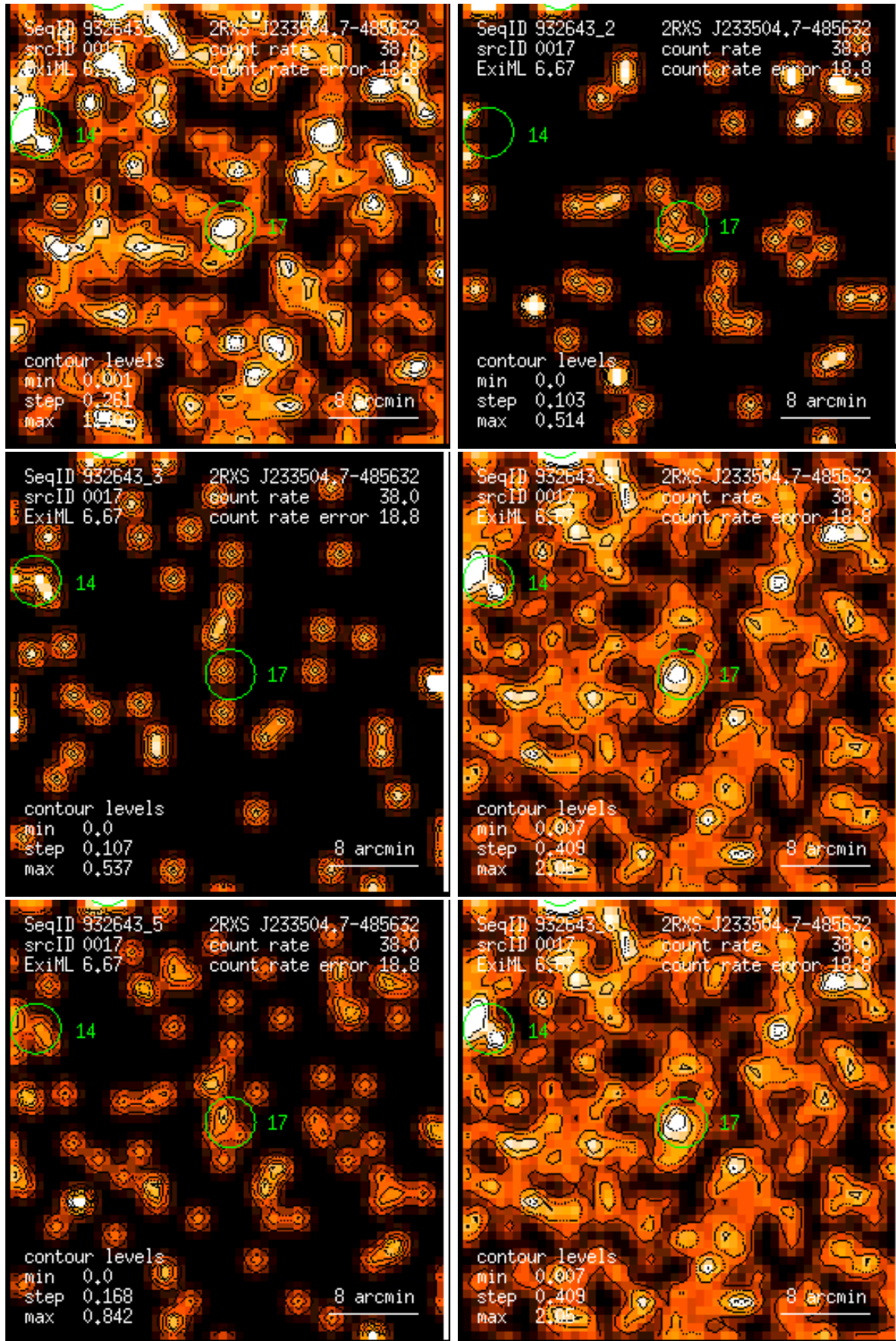
Figure 17: RASS 932643: detection 0017: band rate images, Gaussian filter: (1) PSPC channels 11 – 41, (2) 52 – 90, (3) 91 – 201, (4) 11 – 235, (5) 52 – 201, (6) 11 – 201. Broad band rates in counts/ks. Band rate contour levels in counts/ks/arcmin 2 .
