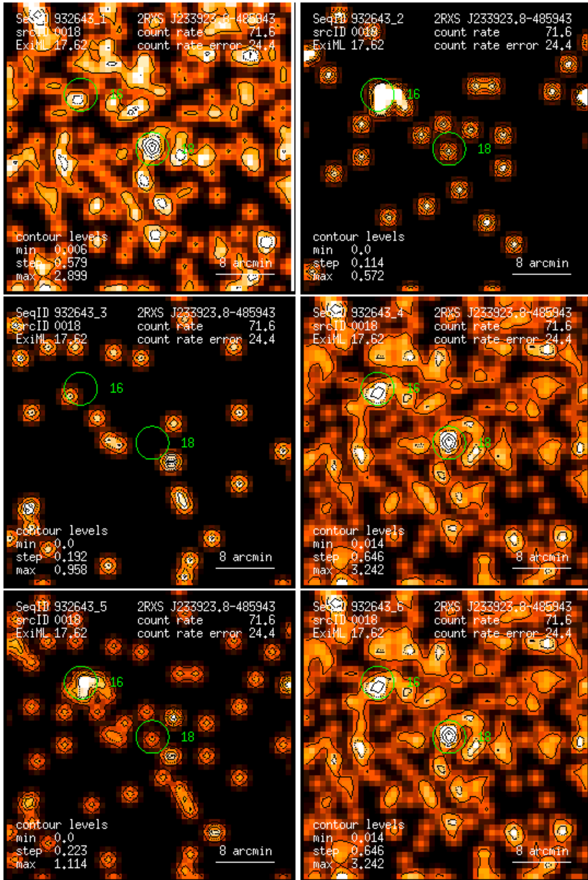
Figure 18: RASS 932643: detection 0018: band rate images, Gaussian filter: (1) PSPC channels 11 – 41, (2) 52 – 90, (3) 91 – 201, (4) 11 – 235, (5) 52 – 201, (6) 11 – 201. Broad band rates in counts/ks. Band rate contour levels in counts/ks/arcmin 2 .
