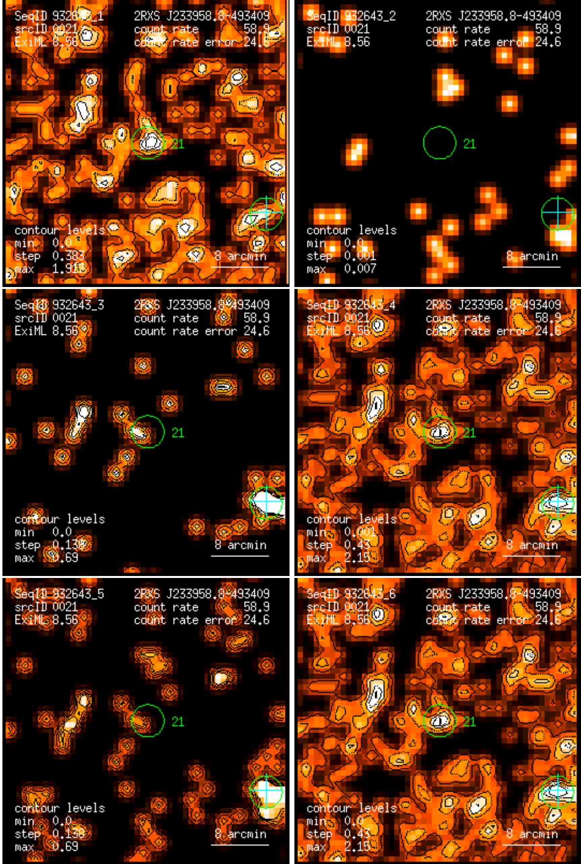
Figure 21: RASS 932643: detection 0021: band rate images, Gaussian filter: (1) PSPC channels 11 – 41, (2) 52 – 90, (3) 91 – 201, (4) 11 – 235, (5) 52 – 201, (6) 11 – 201. Broad band rates in counts/ks. Band rate contour levels in counts/ks/arcmin 2 .
