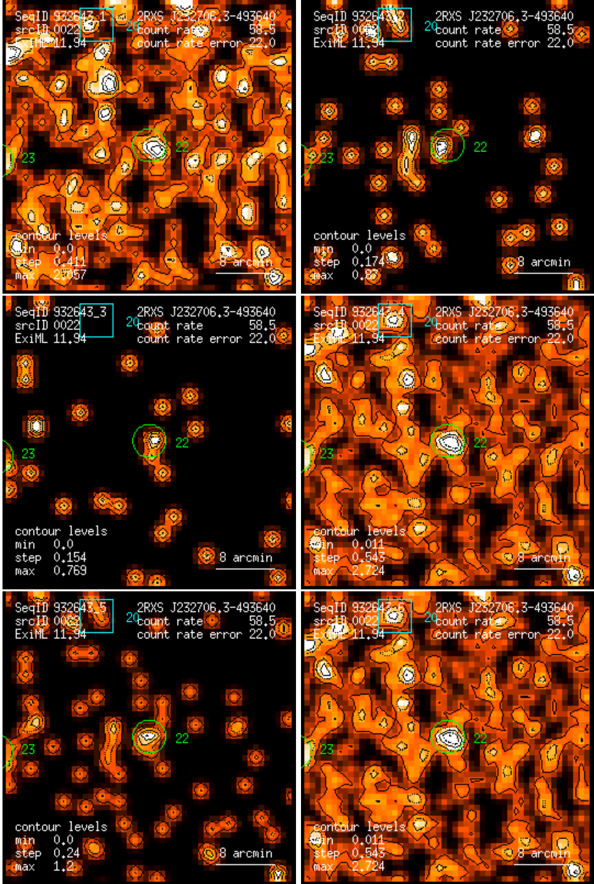
Figure 22: RASS 932643: detection 0022: band rate images, Gaussian filter: (1) PSPC channels 11 – 41, (2) 52 – 90, (3) 91 – 201, (4) 11 – 235, (5) 52 – 201, (6) 11 – 201. Broad band rates in counts/ks. Band rate contour levels in counts/ks/arcmin 2 .
