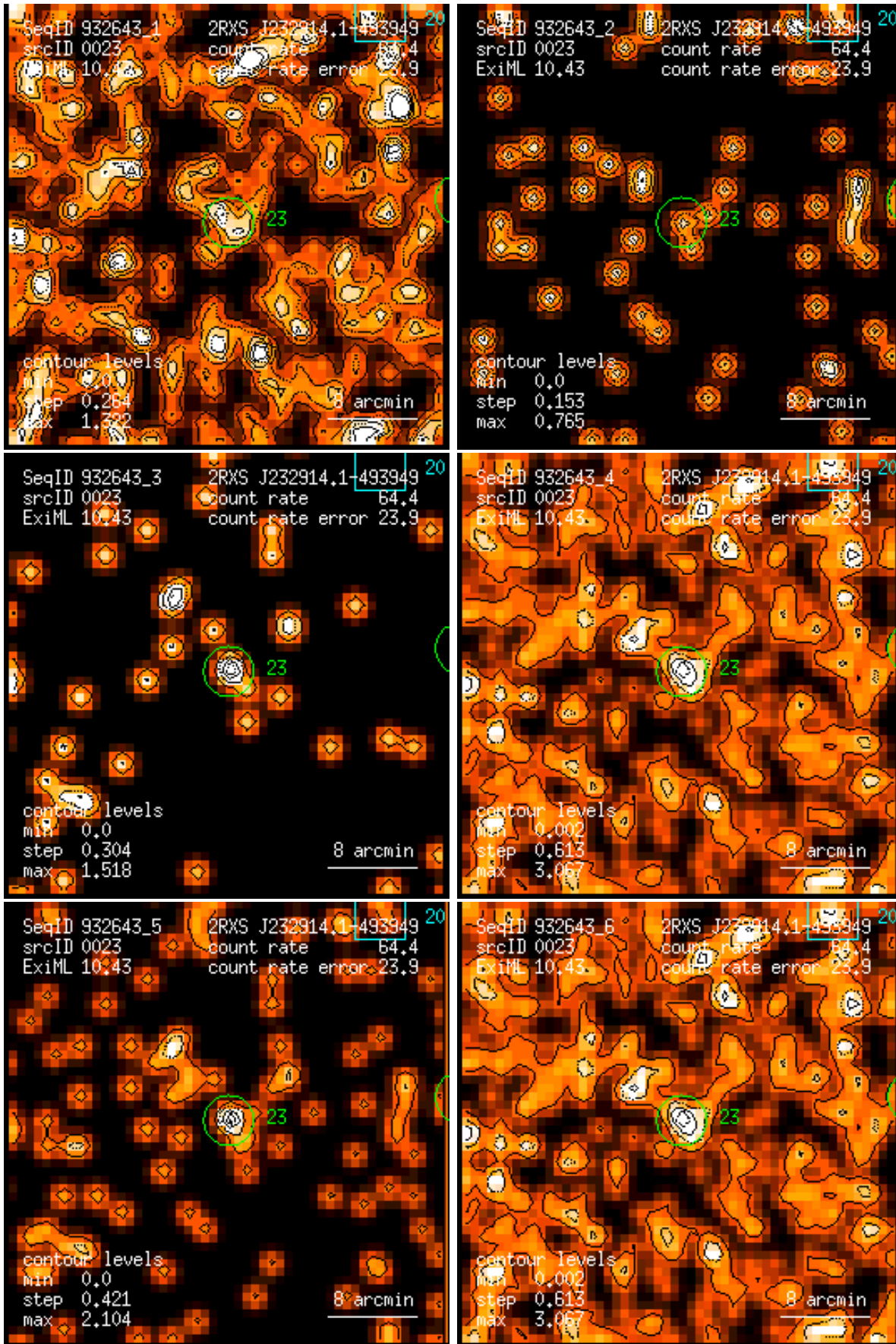
Figure 23: RASS 932643: detection 0023: band rate images, Gaussian filter: (1) PSPC channels 11 – 41, (2) 52 – 90, (3) 91 – 201, (4) 11 – 235, (5) 52 – 201, (6) 11 – 201. Broad band rates in counts/ks. Band rate contour levels in counts/ks/arcmin 2 .
