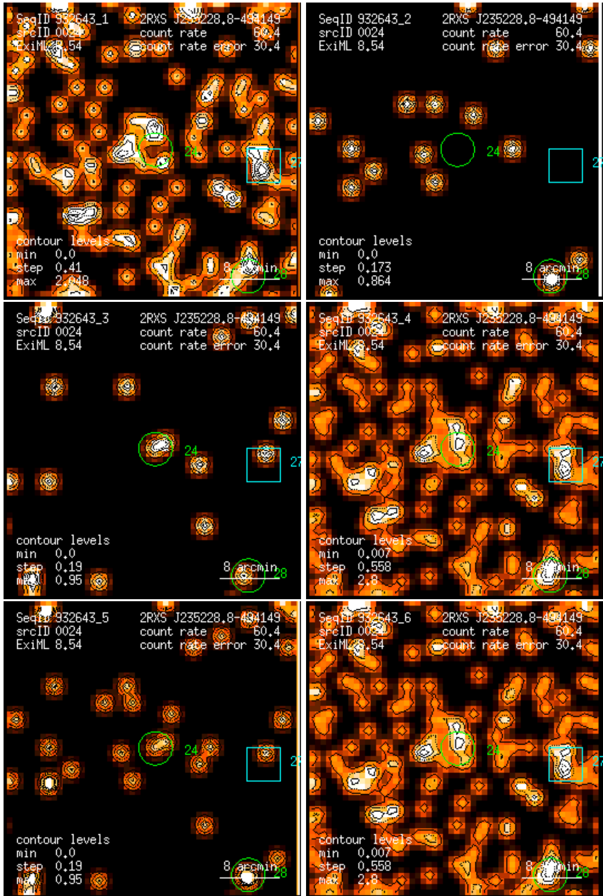
Figure 24: RASS 932643: detection 0024: band rate images, Gaussian filter: (1) PSPC channels 11 – 41, (2) 52 – 90, (3) 91 – 201, (4) 11 – 235, (5) 52 – 201, (6) 11 – 201. Broad band rates in counts/ks. Band rate contour levels in counts/ks/arcmin 2 .
