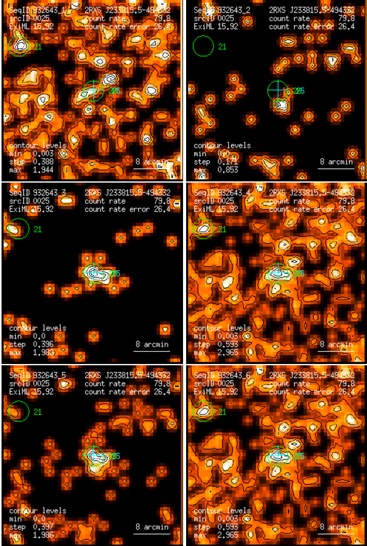
Figure 25: RASS 932643: detection 0025: band rate images, Gaussian filter: (1) PSPC channels 11 – 41, (2) 52 – 90, (3) 91 – 201, (4) 11 – 235, (5) 52 – 201, (6) 11 – 201. Broad band rates in counts/ks. Band rate contour levels in counts/ks/arcmin 2 .
