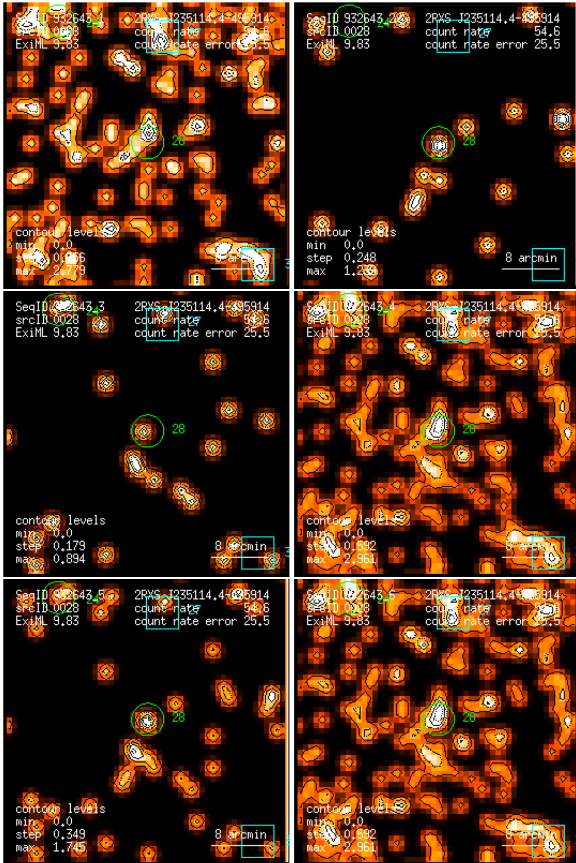
Figure 28: RASS 932643: detection 0028: band rate images, Gaussian filter: (1) PSPC channels 11 – 41, (2) 52 – 90, (3) 91 – 201, (4) 11 – 235, (5) 52 – 201, (6) 11 – 201. Broad band rates in counts/ks. Band rate contour levels in counts/ks/arcmin 2 .
