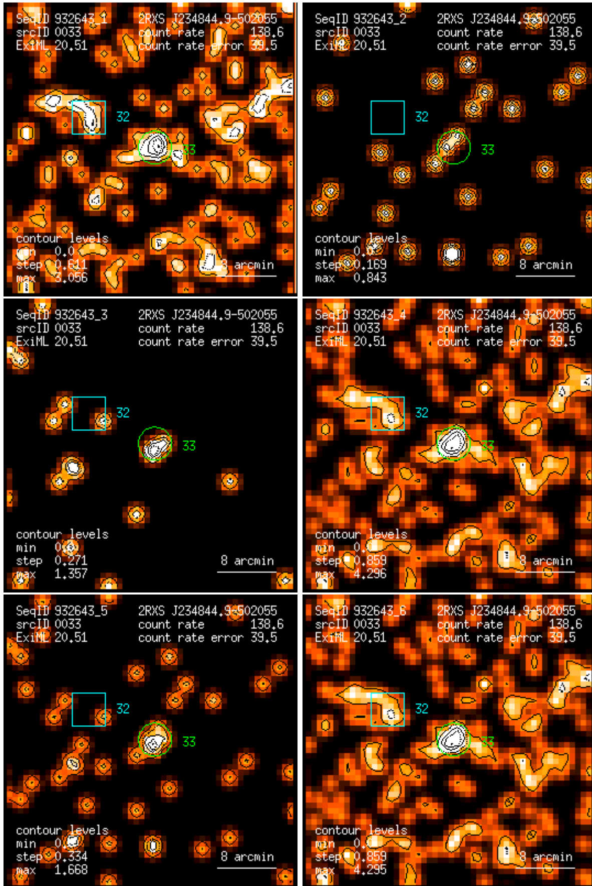
Figure 33: RASS 932643: detection 0033: band rate images, Gaussian filter: (1) PSPC channels 11 – 41, (2) 52 – 90, (3) 91 – 201, (4) 11 – 235, (5) 52 – 201, (6) 11 – 201. Broad band rates in counts/ks. Band rate contour levels in counts/ks/arcmin 2 .
