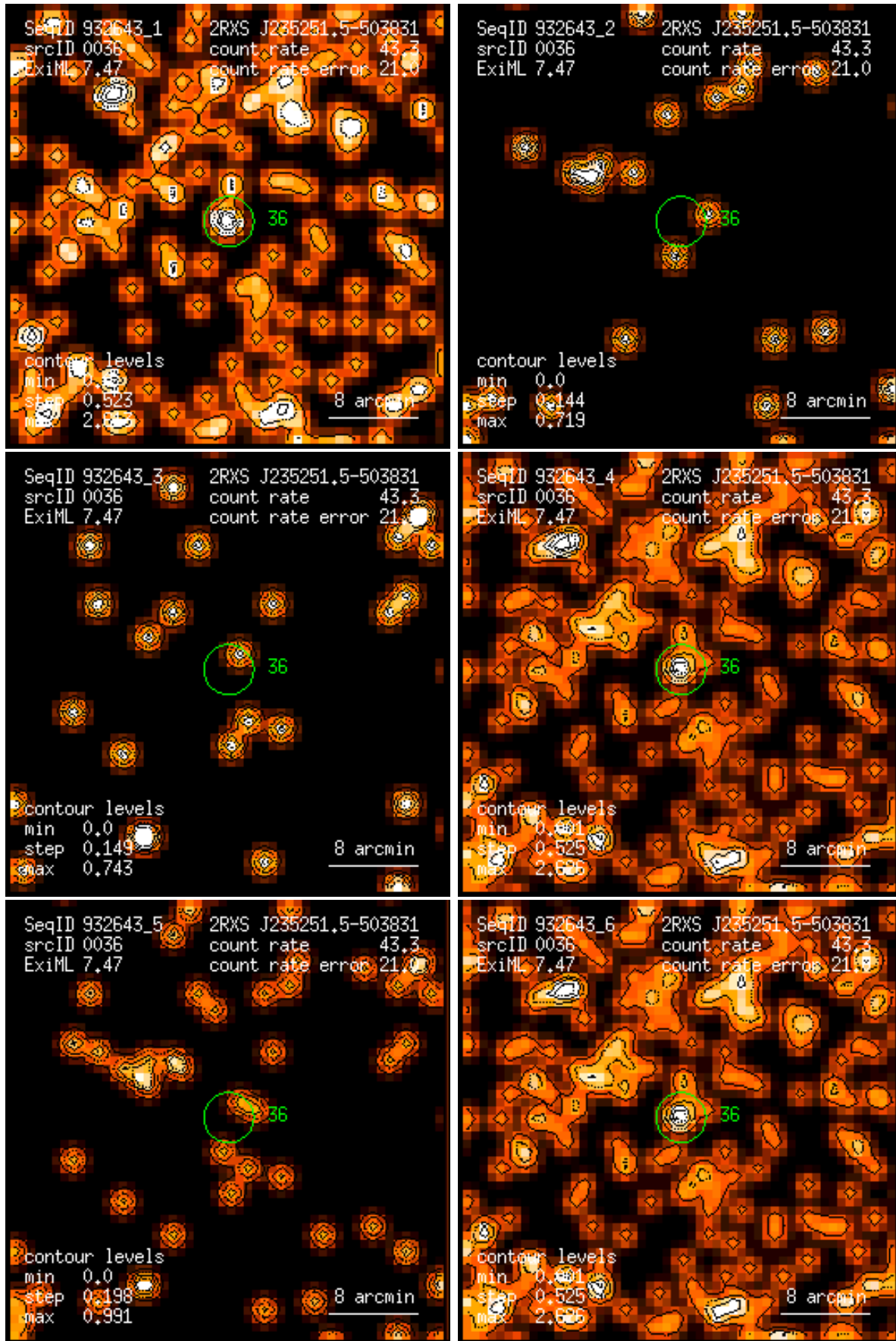
Figure 36: RASS 932643: detection 0036: band rate images, Gaussian filter: (1) PSPC channels 11 – 41, (2) 52 – 90, (3) 91 – 201, (4) 11 – 235, (5) 52 – 201, (6) 11 – 201. Broad band rates in counts/ks. Band rate contour levels in counts/ks/arcmin 2 .
