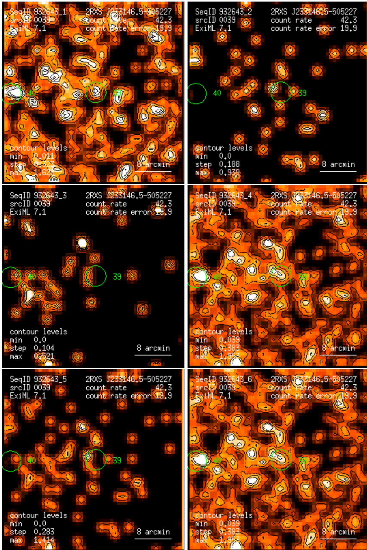
Figure 39: RASS 932643: detection 0039: band rate images, Gaussian filter: (1) PSPC channels 11 – 41, (2) 52 – 90, (3) 91 – 201, (4) 11 – 235, (5) 52 – 201, (6) 11 – 201. Broad band rates in counts/ks. Band rate contour levels in counts/ks/arcmin 2 .
