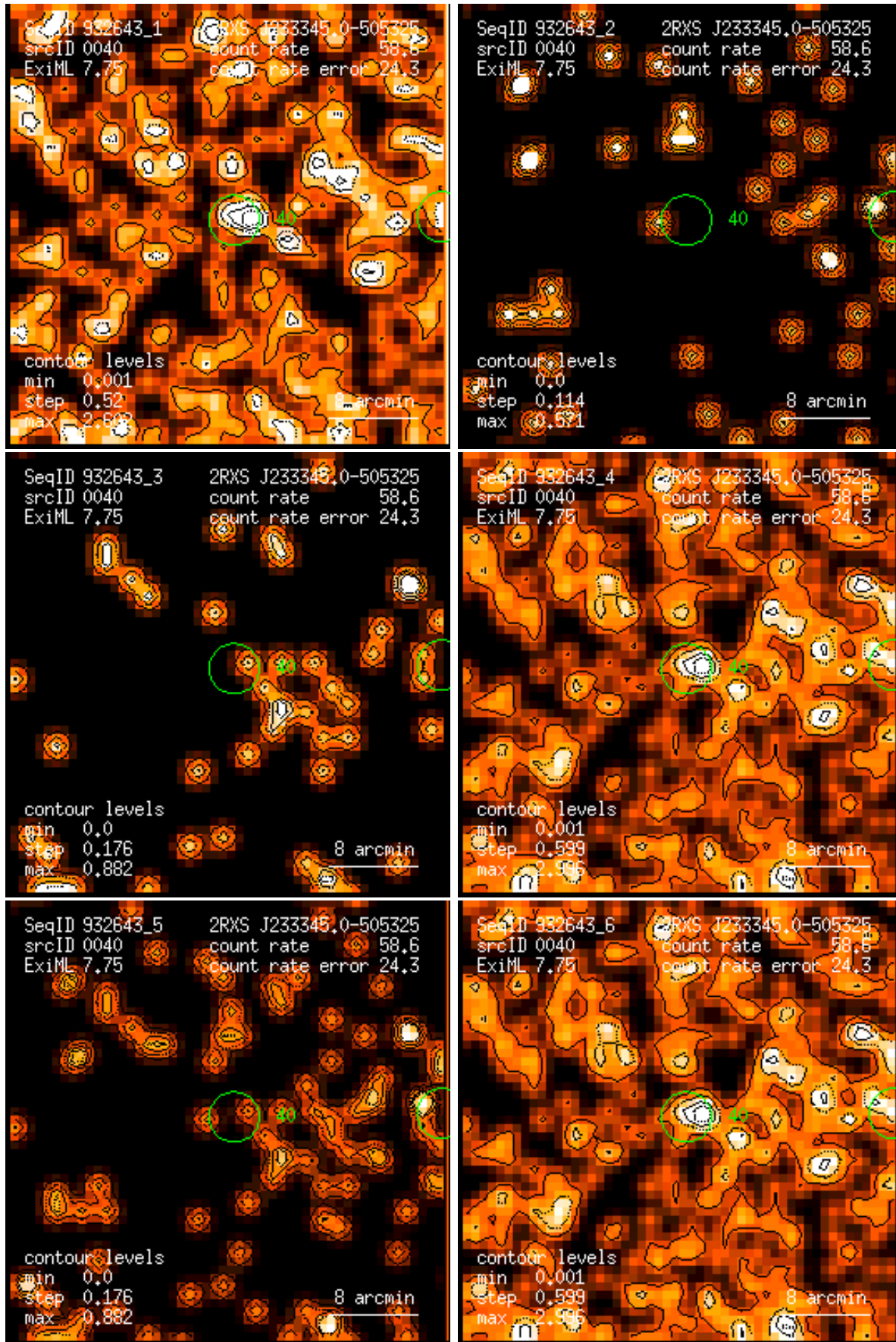
Figure 40: RASS 932643: detection 0040: band rate images, Gaussian filter: (1) PSPC channels 11 – 41, (2) 52 – 90, (3) 91 – 201, (4) 11 – 235, (5) 52 – 201, (6) 11 – 201. Broad band rates in counts/ks. Band rate contour levels in counts/ks/arcmin 2 .
