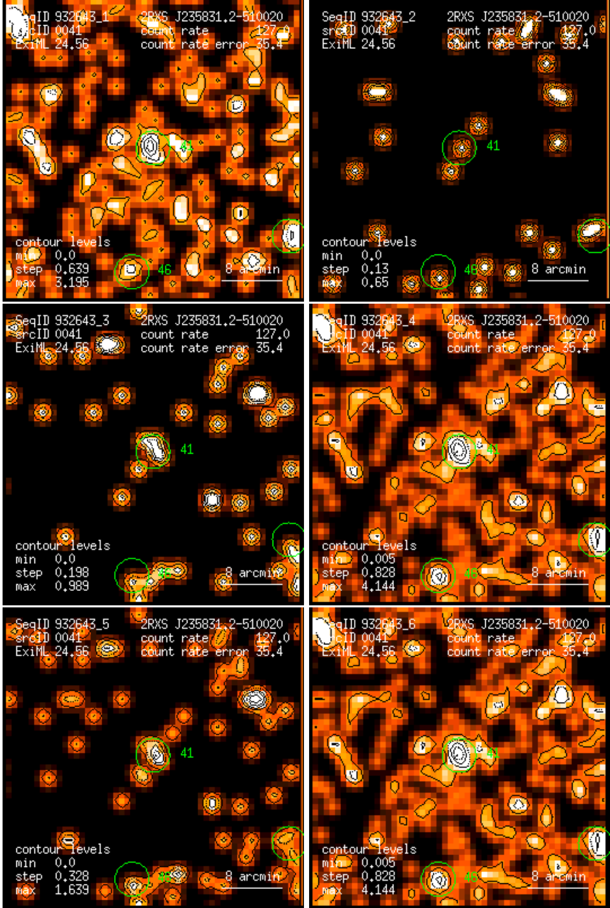
Figure 41: RASS 932643: detection 0041: band rate images, Gaussian filter: (1) PSPC channels 11 – 41, (2) 52 – 90, (3) 91 – 201, (4) 11 – 235, (5) 52 – 201, (6) 11 – 201. Broad band rates in counts/ks. Band rate contour levels in counts/ks/arcmin 2 .
