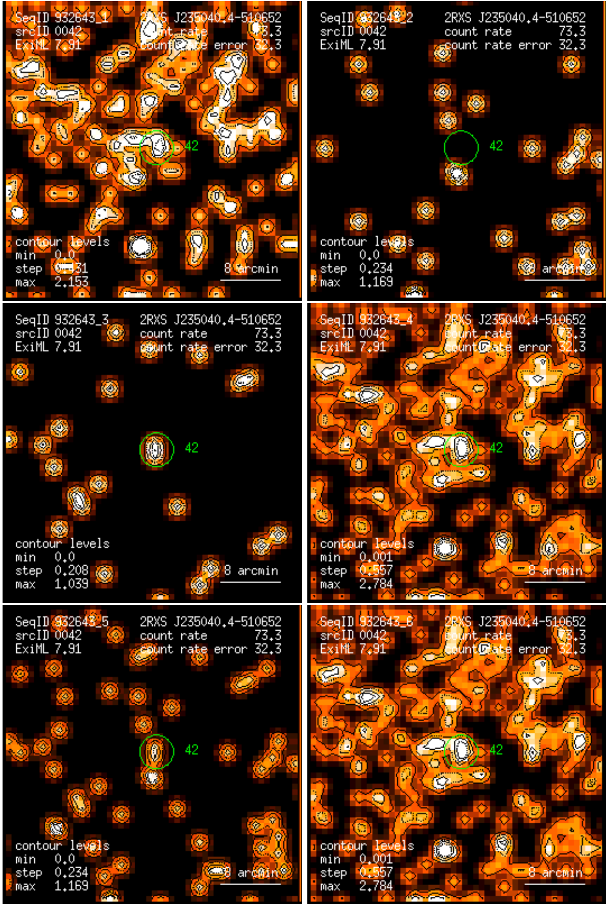
Figure 42: RASS 932643: detection 0042: band rate images, Gaussian filter: (1) PSPC channels 11 – 41, (2) 52 – 90, (3) 91 – 201, (4) 11 – 235, (5) 52 – 201, (6) 11 – 201. Broad band rates in counts/ks. Band rate contour levels in counts/ks/arcmin 2 .
