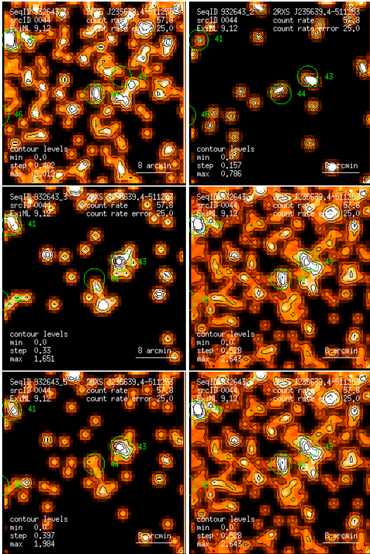
Figure 44: RASS 932643: detection 0044: band rate images, Gaussian filter: (1) PSPC channels 11 – 41, (2) 52 – 90, (3) 91 – 201, (4) 11 – 235, (5) 52 – 201, (6) 11 – 201. Broad band rates in counts/ks. Band rate contour levels in counts/ks/arcmin 2 .
